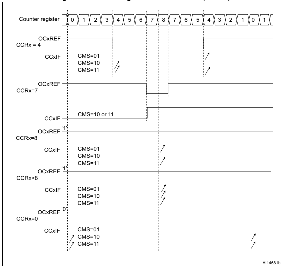
Figure 103. Center-aligned PWM waveforms (ARR=8)
