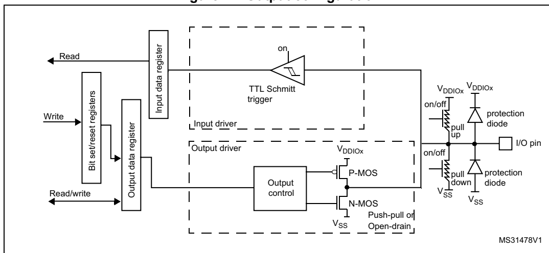
Figure 22. Output configuration
