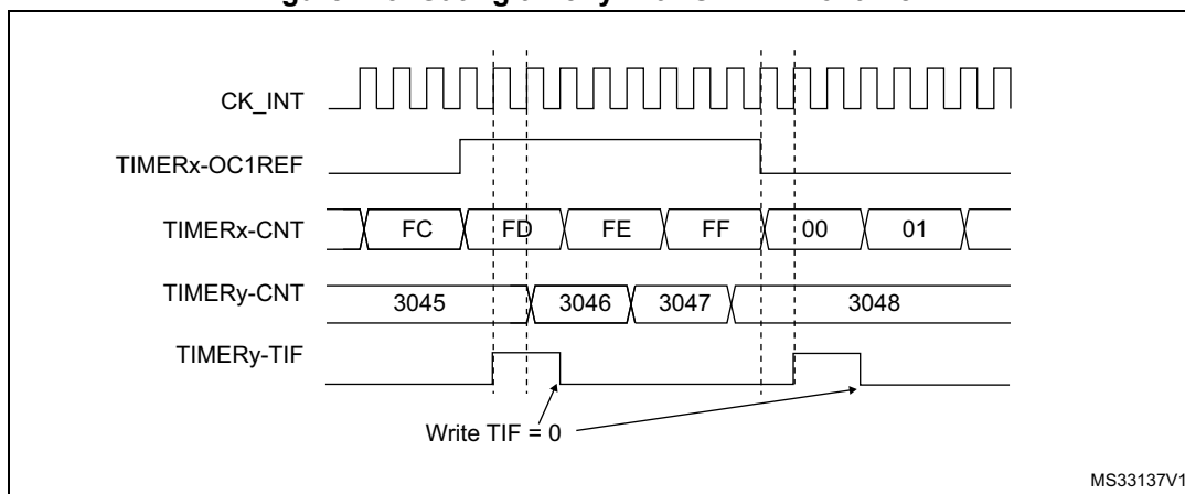
Figure 113. Gating timer y with OC1REF of timer x
