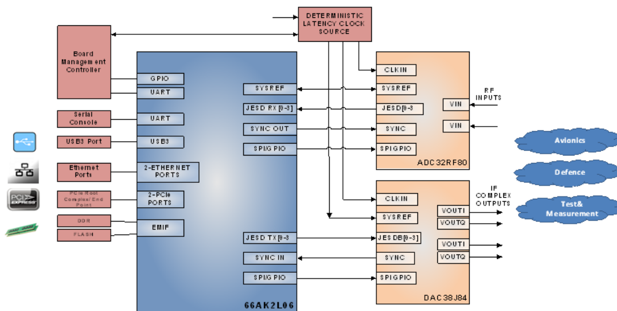
Figure 3. Block Diagram
