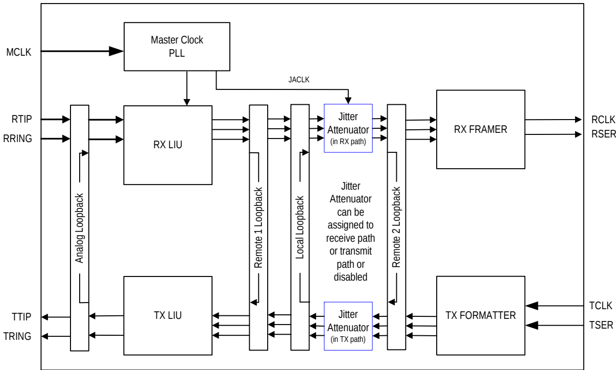
Figure 9-27. Loopback Diagram
