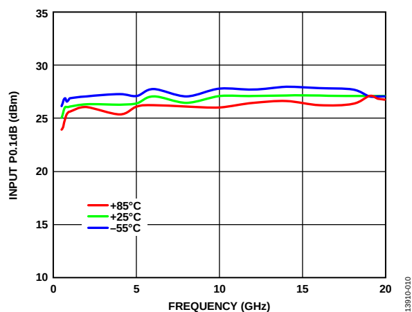
Figure 10. Input Power 0.1 dB vs. Frequency over Temperature, V_{CTL} = -5\text{ V}
