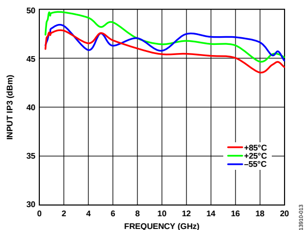
Figure 11. Input IP3 vs. Frequency over Temperature, V_{CTL} = -5\text{ V}
