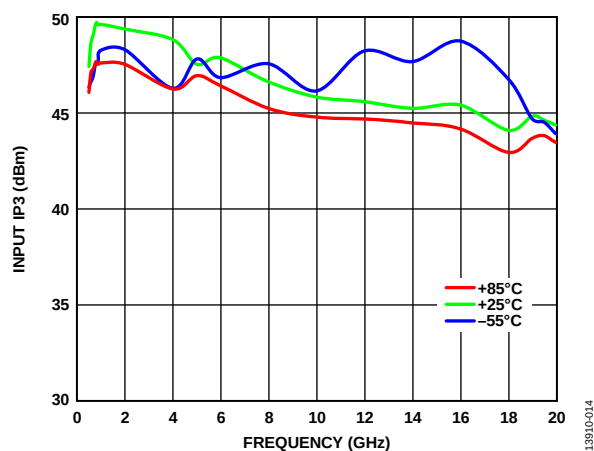
Figure 12. Input IP3 vs. Frequency over Temperature, V_{CTL} = -3\text{ V}
