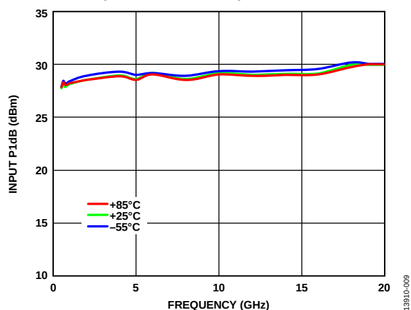
Figure 9. Input P1dB vs. Frequency over Temperature, V_{CTL} = -5\text{ V}
