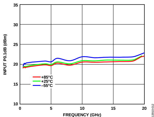
Figure 11. Input P0.1dB vs. Frequency over Temperature, V_{CTL} = -3\text{ V}
