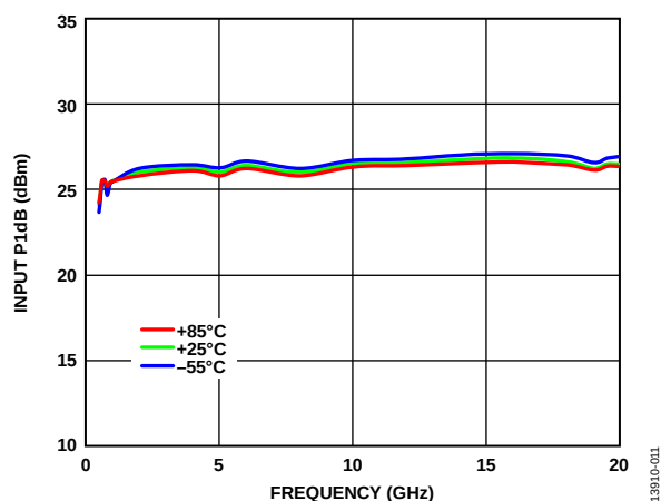
Figure 10. Input P1dB vs. Frequency over Temperature, V_{CTL} = -3\text{ V}
