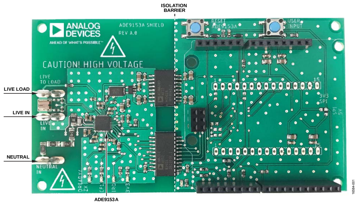
Figure 1. EV-ADE9153ASHIELDZ Connection Diagram
