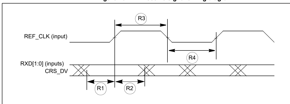
Figure 40. RMII receive signal timing diagram
