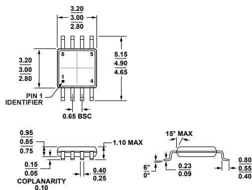
Figure 44. 8-Lead Mini Small Outline Package [MSOP] (RM-8)
