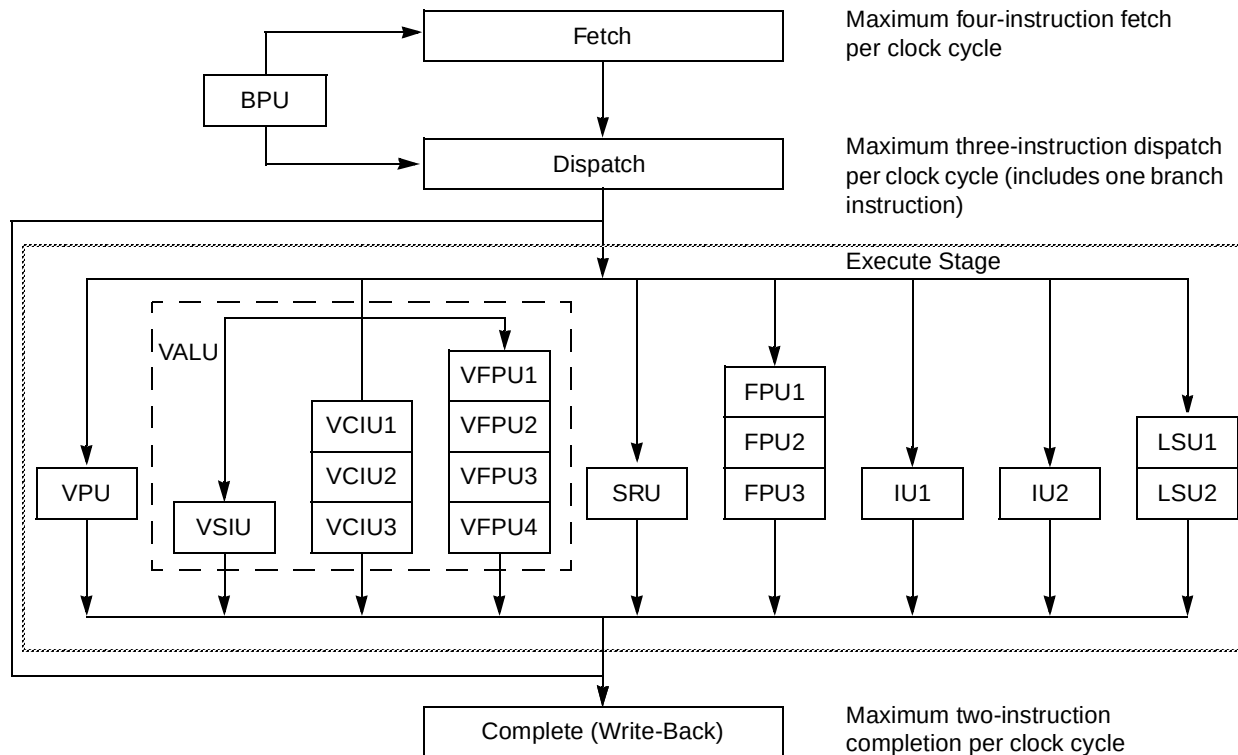
Figure 1-6. Pipeline Diagram
