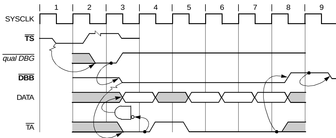
Figure 9-11. Read Burst with \overline{\text{TA}} Wait States
