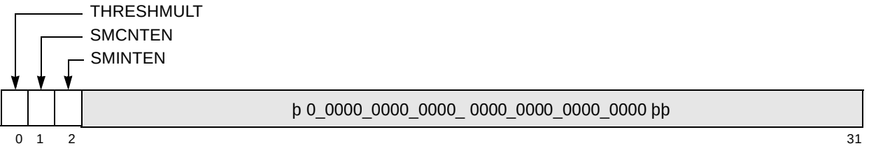
Figure 2-14. Monitor Mode Control Register 2 (MMCR2)
