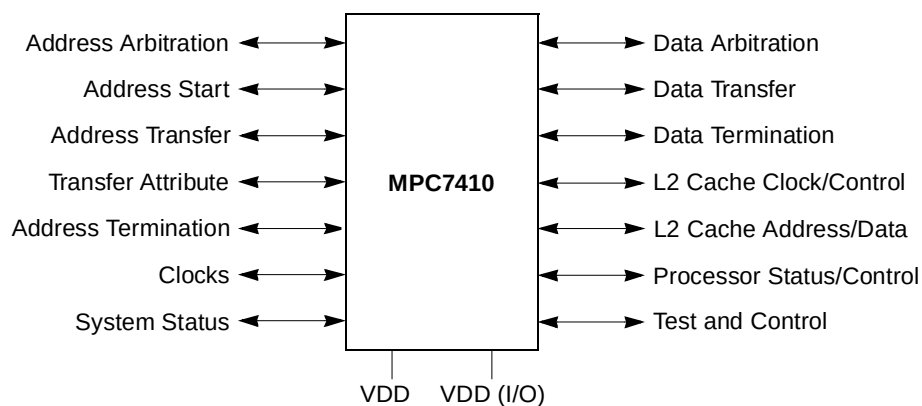
Figure 1-3. System Interface
