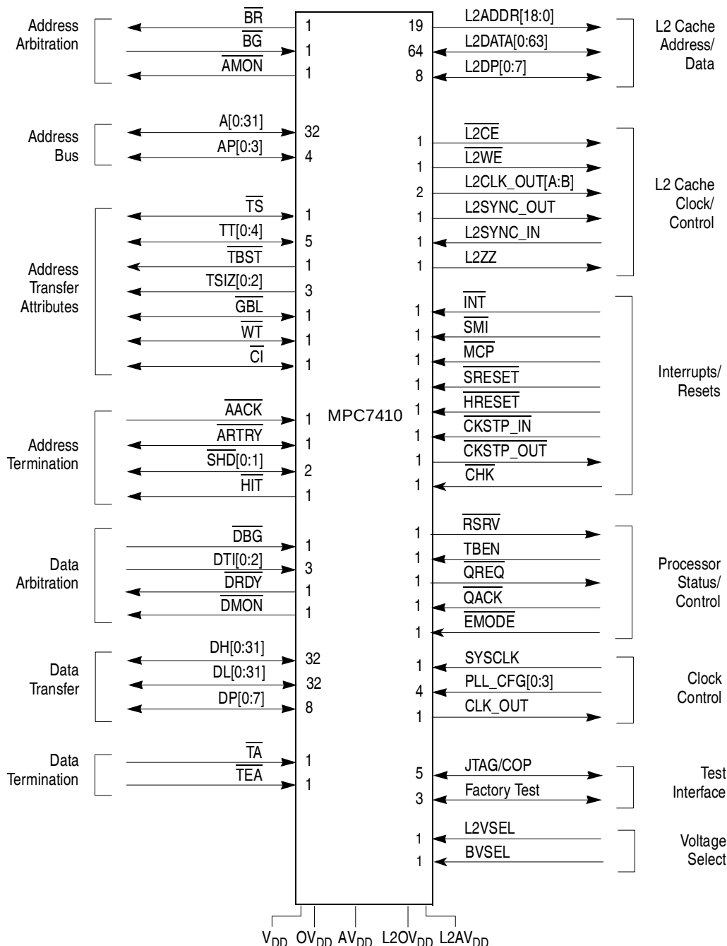
Figure 8-2. MPX Bus Signal Groups
