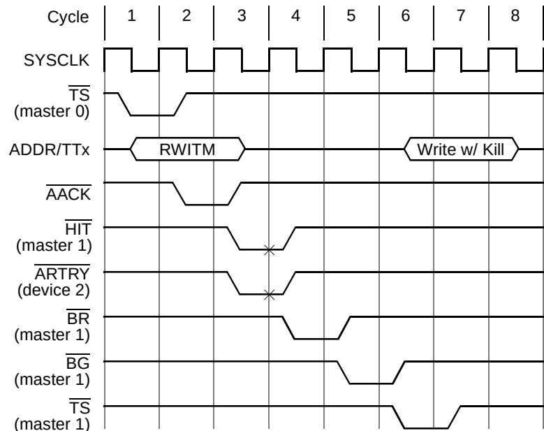
Figure 9-23 shows an example timing diagram of \overline{\text{HIT}} and \overline{\text{ARTRY}} being asserted together.
