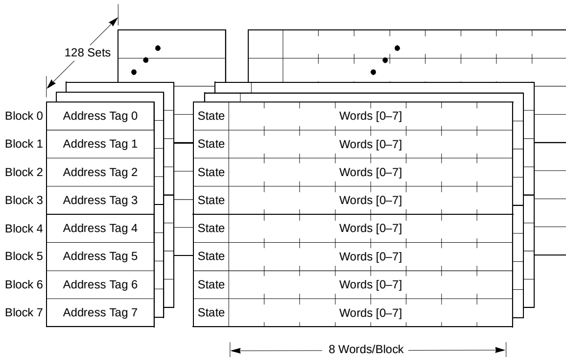
Figure 1-2. L1 Cache Organization
