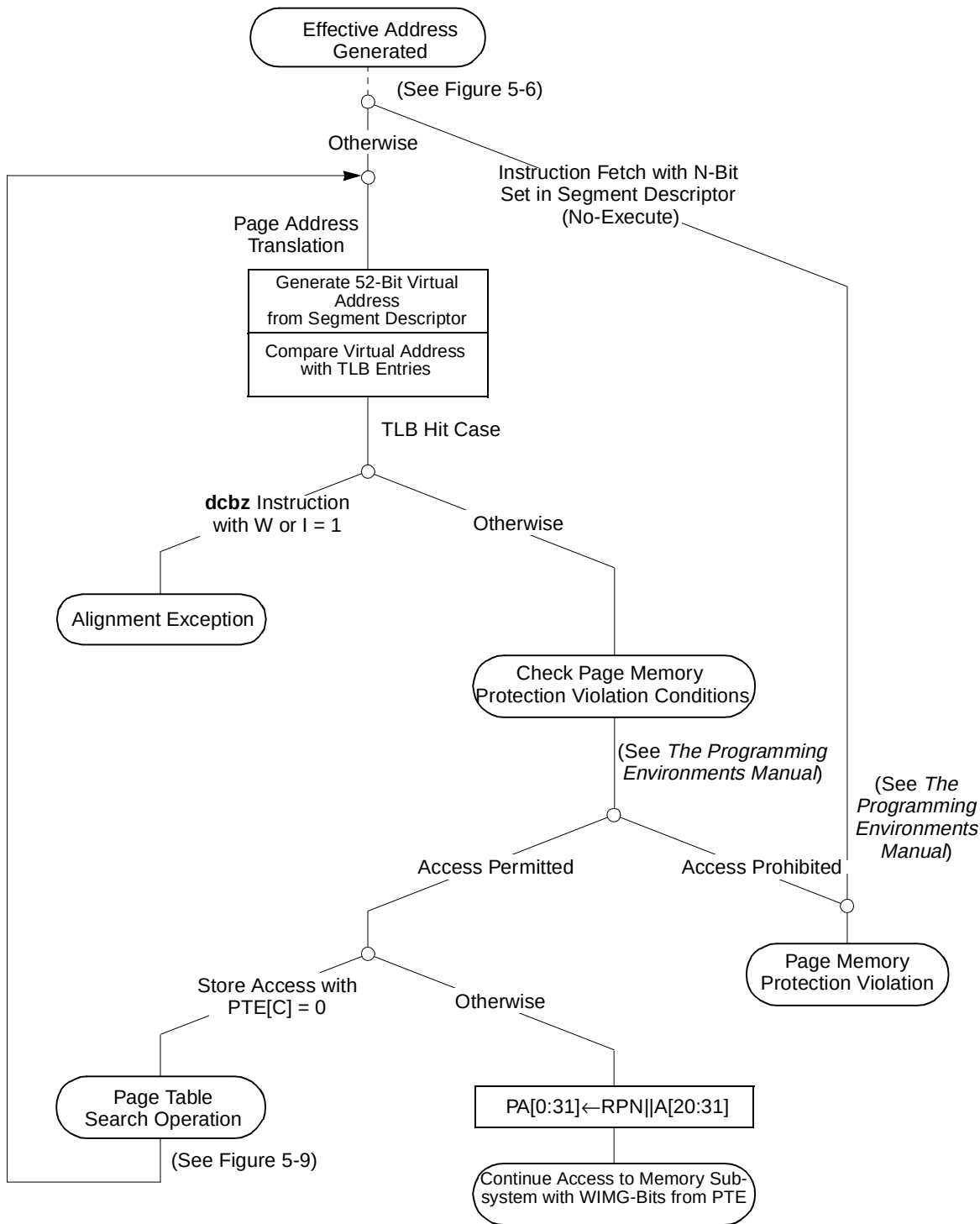
Figure 5-10. Page Address Translation Flow—TLB Hit
