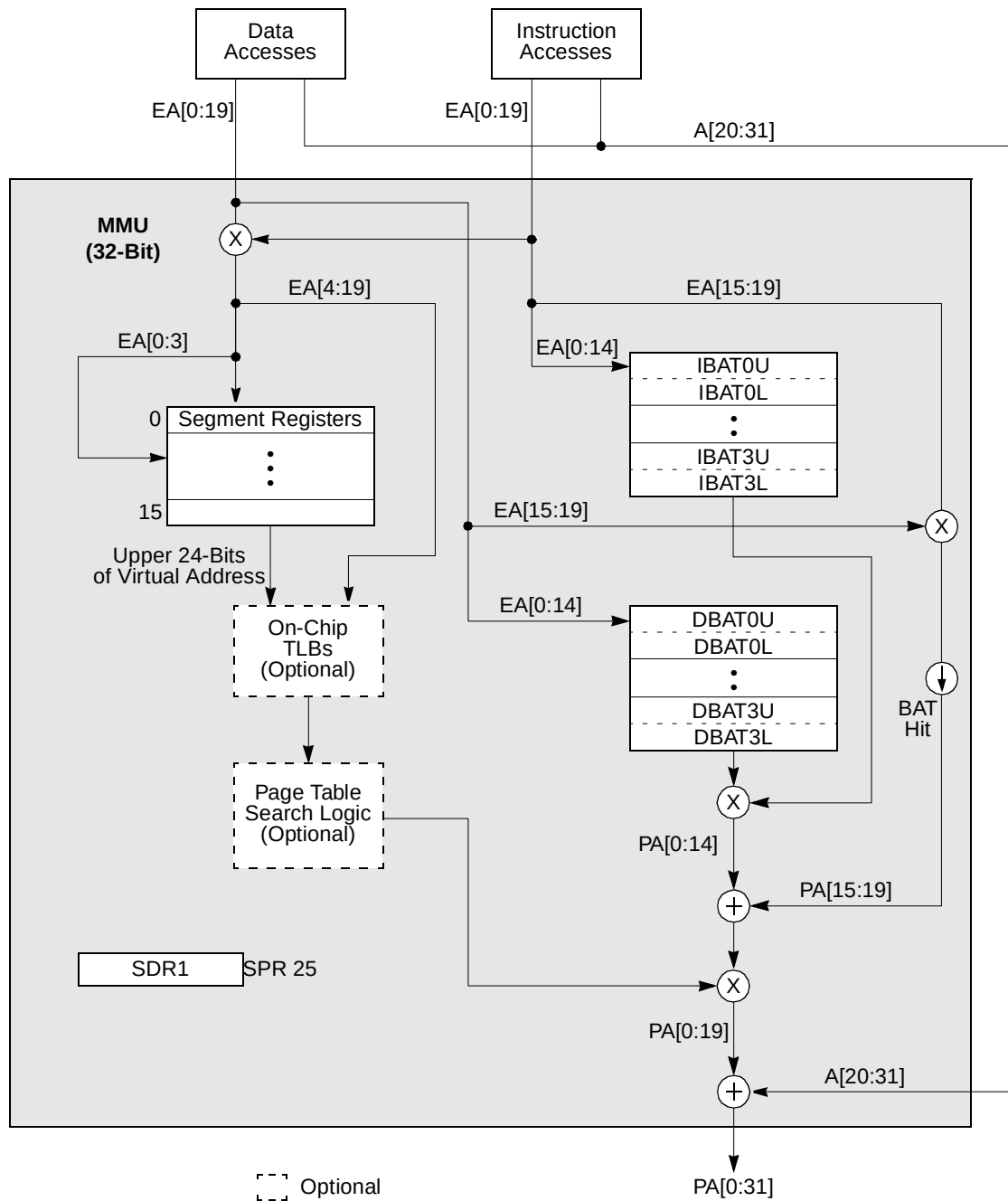
Figure 5-1. MMU Conceptual Block Diagram—32-Bit Implementations
