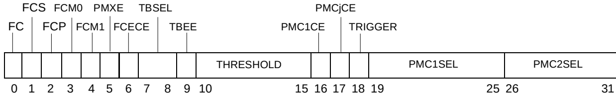
Figure 2-12. Monitor Mode Control Register 0 (MMCR0)
