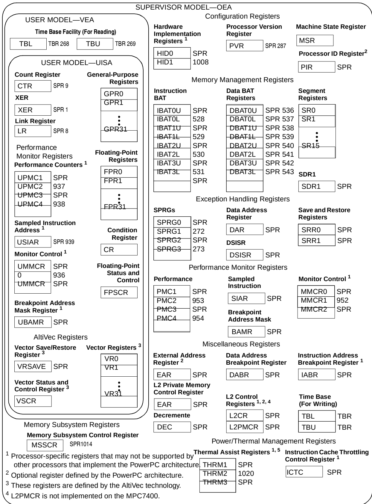
Figure 1-5. MPC7410 Microprocessor Programming Model—Registers
