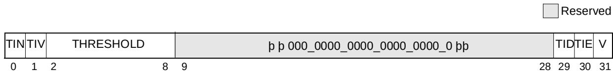
Figure 2-9. Thermal Management Registers 1–2 (THRM1–THRM2)—MPC7400 Only
