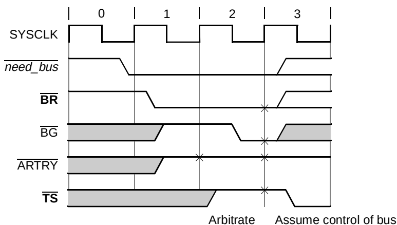
Figure 9-18. MPX Bus Address Bus Arbitration—Non-Parked Case
