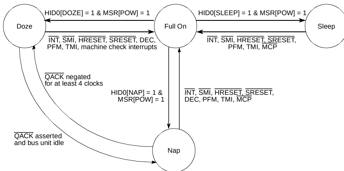
Figure 10-1. Power Management State Diagram
