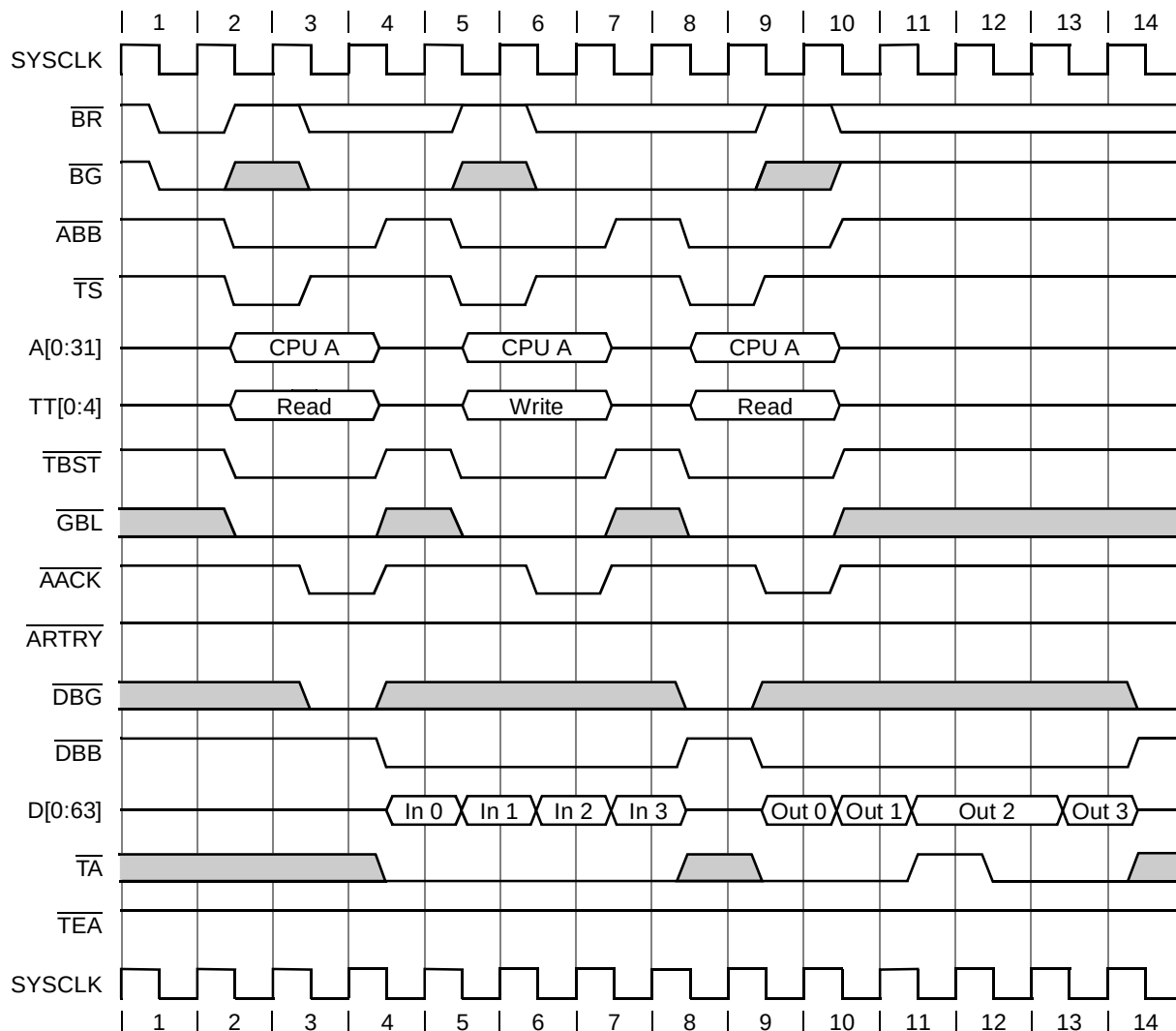
Figure 9-16. Burst Transfers with Data Delay Controls
