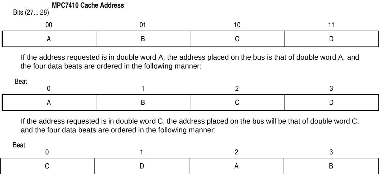
Figure 3-39. Double-Word Address Ordering—Critical Double Word First
