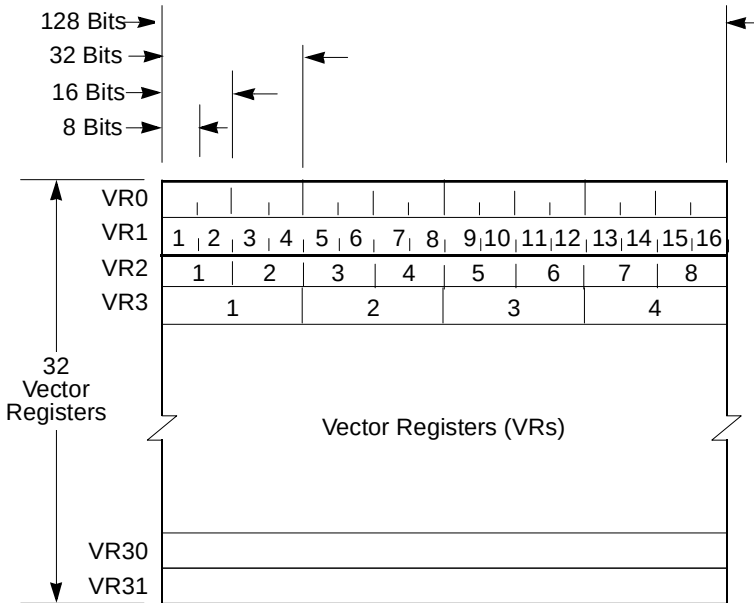
Figure 7-1. Vector Registers (VRs)
