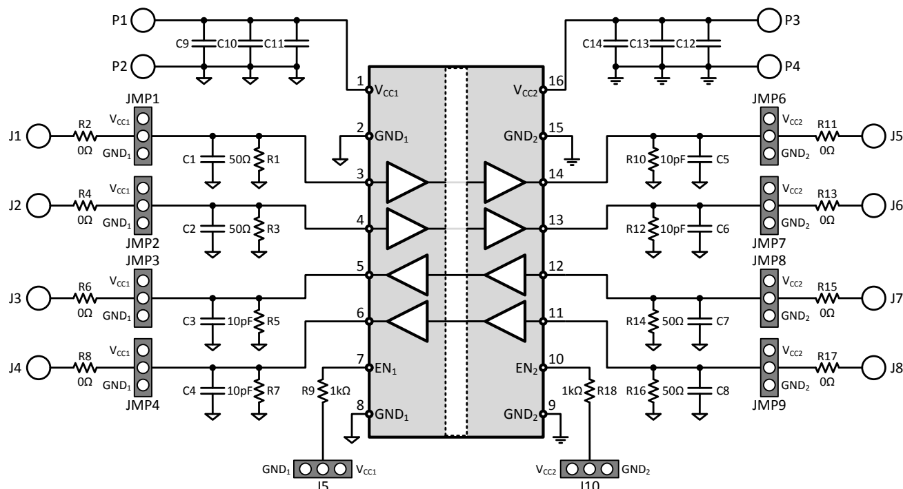
Figure 7. ISO7342x EVM Schematic
