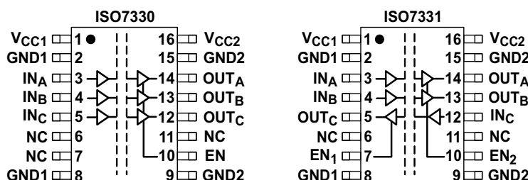
Figure 1. ISO733x Triple-Channel Digital Isolator Pin Configurations
