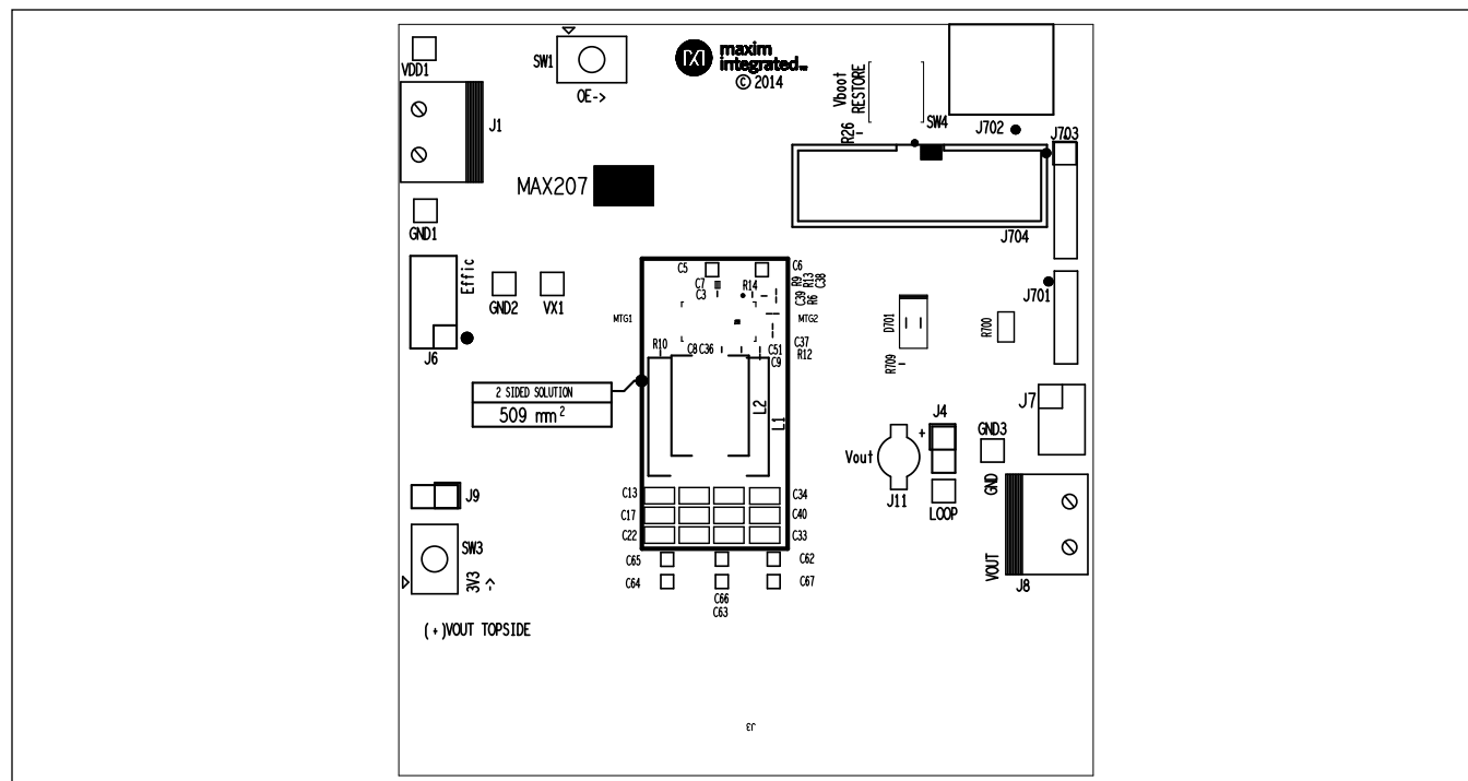
Top Silkscreen
