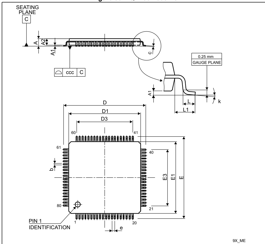
Figure 56. LQFP80 - outline
