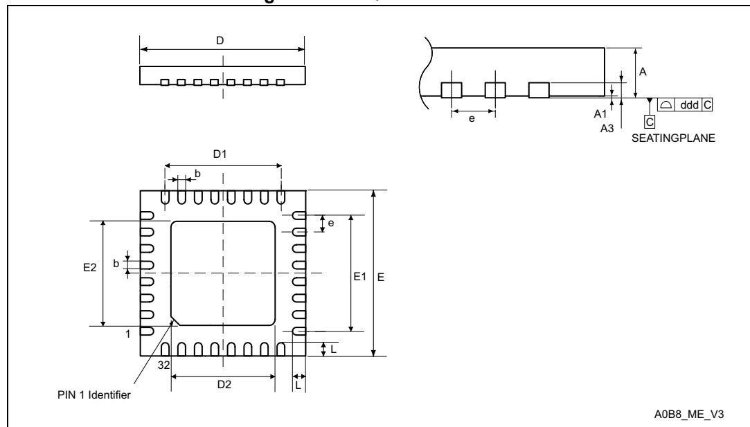
Figure 38. UFQFPN32 - outline
