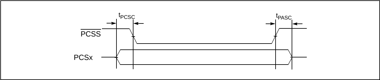
Figure 20. DSPI PCS strobe (PCSS) timing (master mode)
