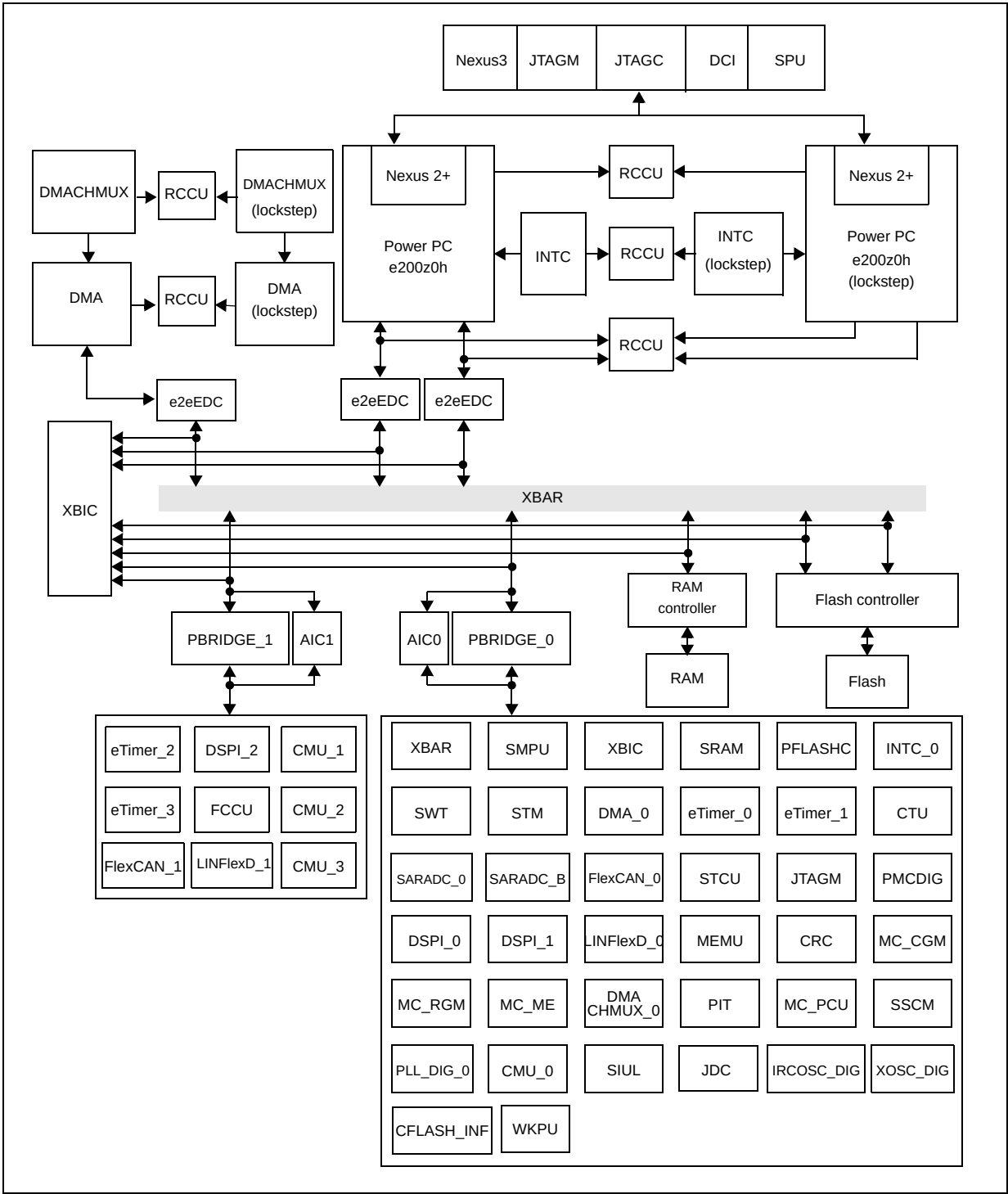
Figure 1. Block diagram
