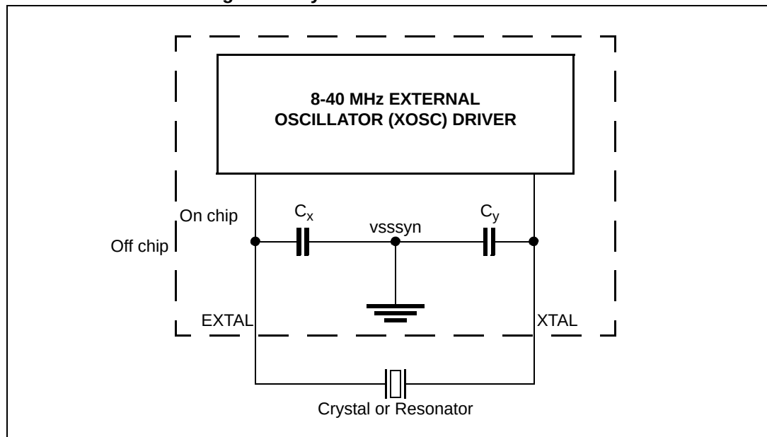
Figure 8. Crystal/Resonator Connections
