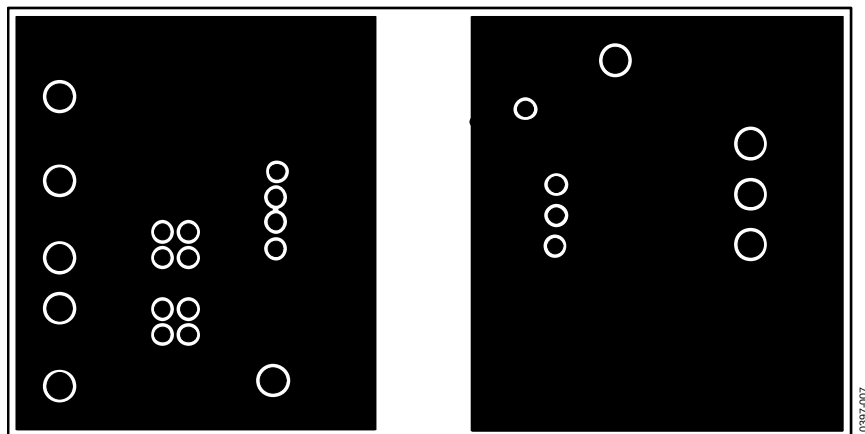
Figure 7. EVAL-ADM3054EBZ Solder Side
