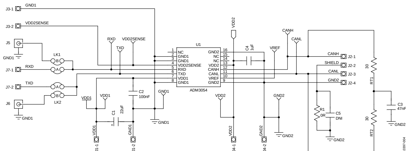
Figure 4. EVAL-ADM3054EBZ Schematic
