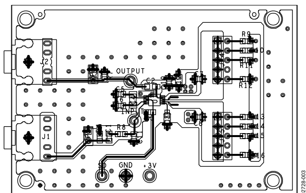
Figure 3. SSM2167 Evaluation Board; Top Layer
