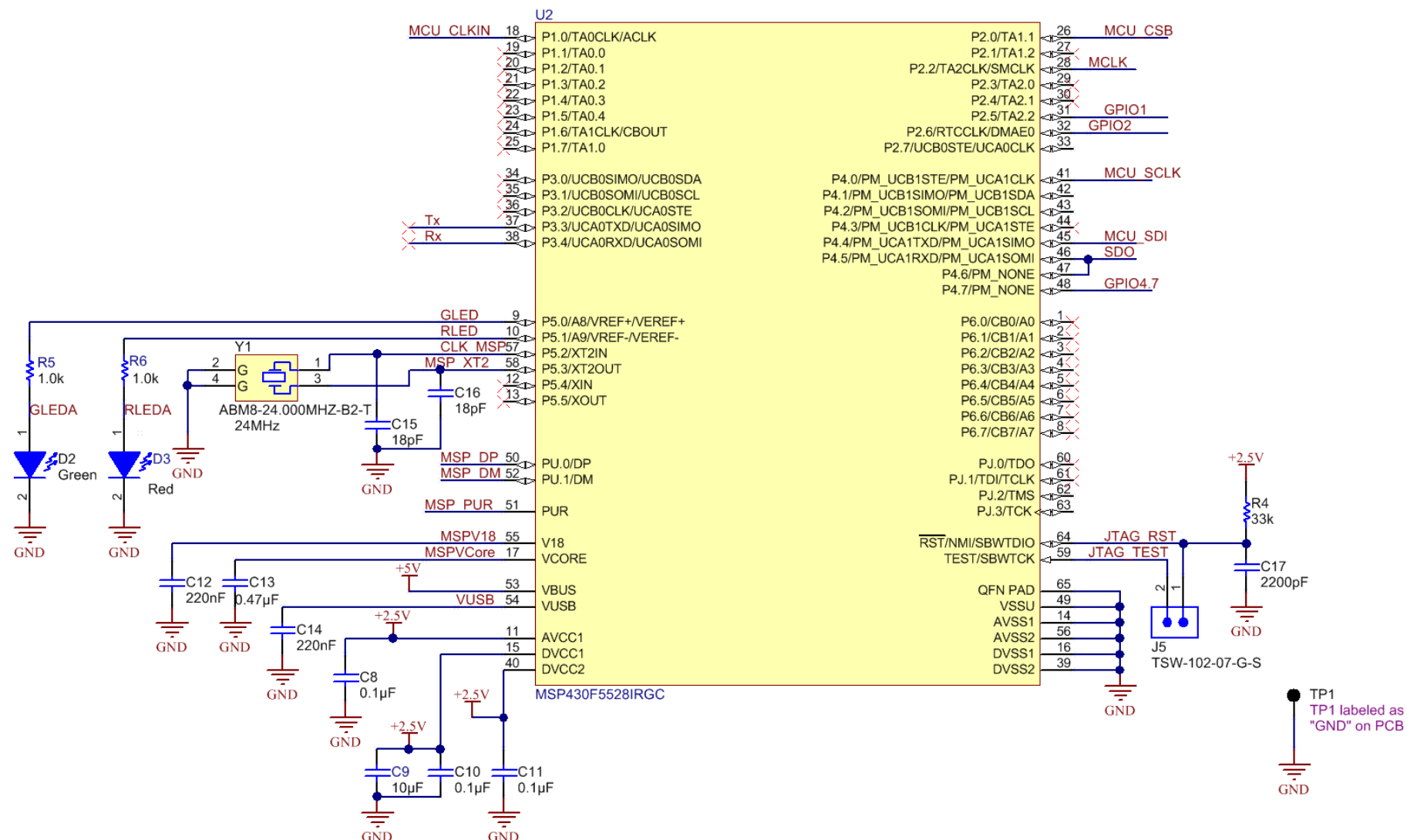
Figure 5-3. MCU Schematic
