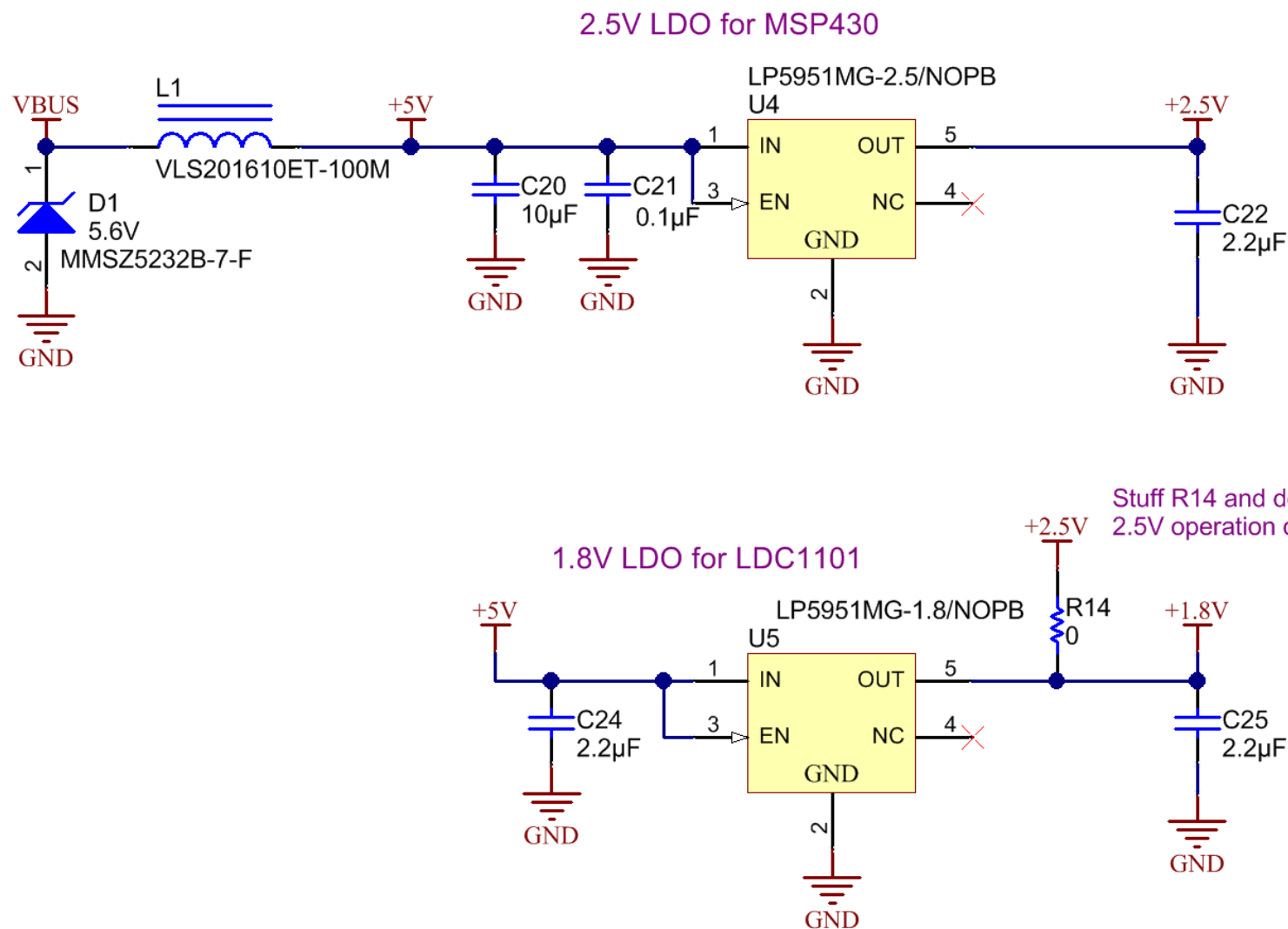
Figure 5-2. Power Conditioning Schematic
