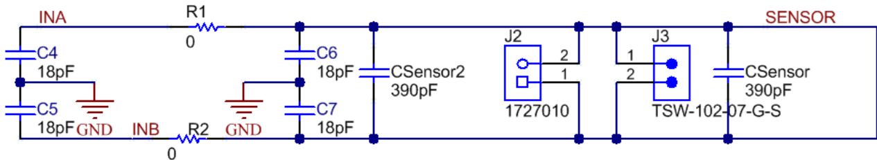
Figure 2-7. Sensor Configuration Options
