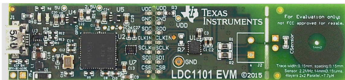
Figure 1-1. LDC1101EVM
