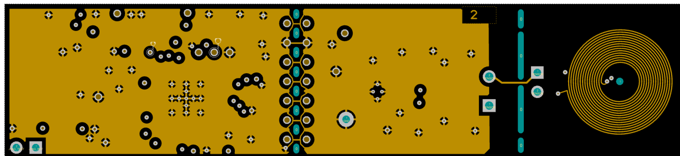
Figure 4-2. Mid-Layer 1 Routing
