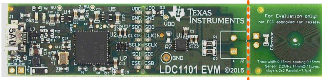
Figure 2-4. Break-Away Sensor
