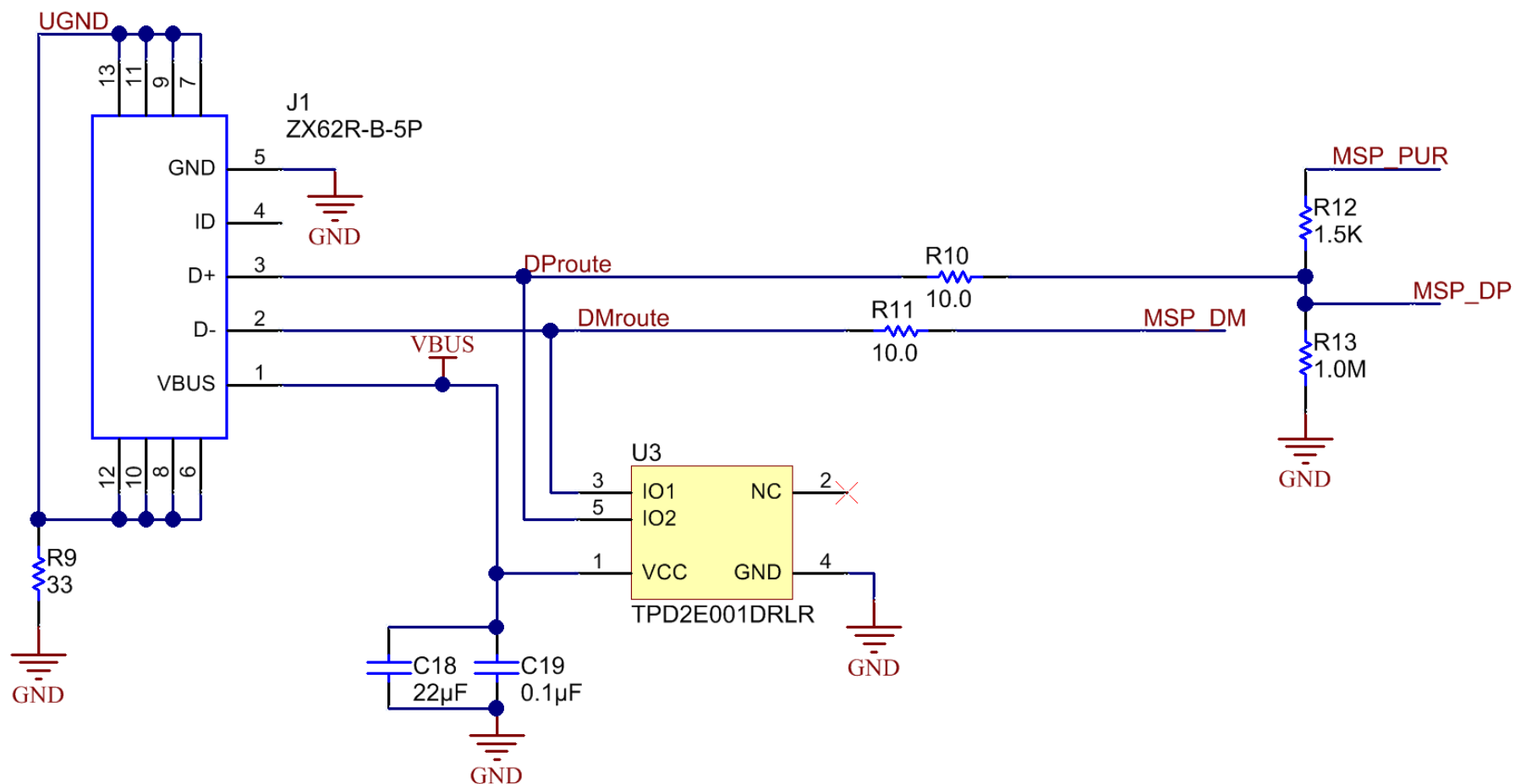
Figure 5-4. USB Connection Schematic
