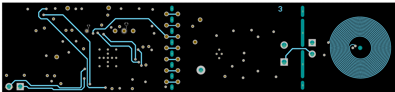
Figure 4-3. Mid-Layer 2 Routing
