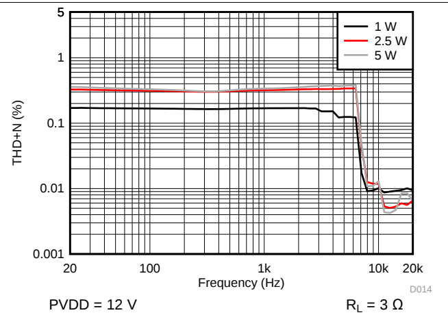
Figure 18. THD+N vs Frequency - PBTL
