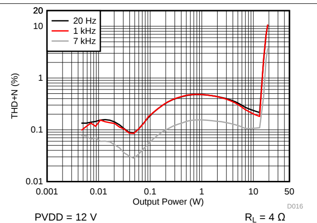
Figure 20. THD+N vs Output Power - PBTL
