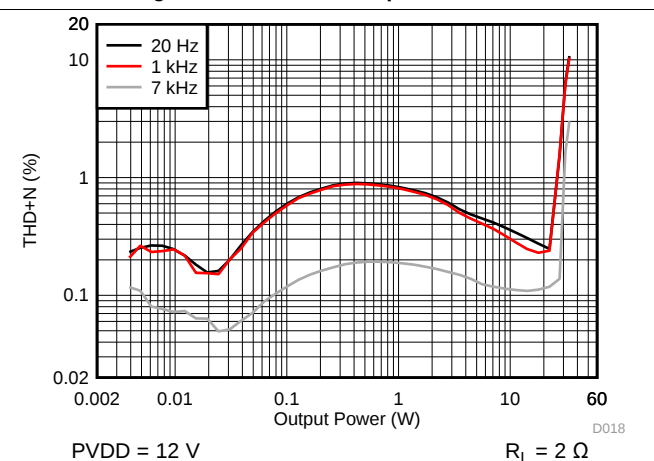
Figure 22. THD+N vs Output Power - PBTL
