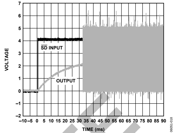
Figure 18. Turn-On Response
