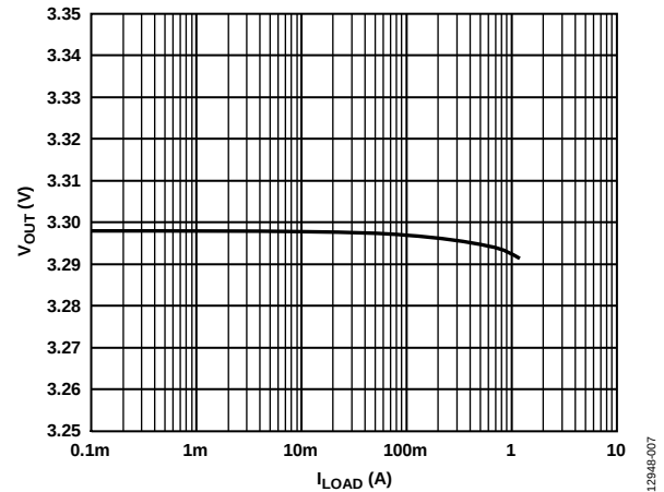
Figure 5. Output Voltage ( V_{OUT} ) vs. Load Current ( I_{LOAD} ), V_{OUT} = 3.3\text{ V} , T_A = 25^\circ\text{C} , C_{IN} = C_{OUT} = 10\text{ }\mu\text{F}
