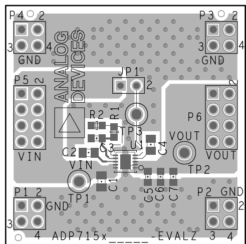
Figure 1. ADP7156CP-3.3EVALZ Printed Circuit Board (PCB) Layout
