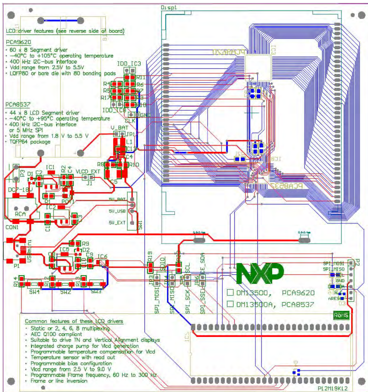
Fig 3. PCB layout
