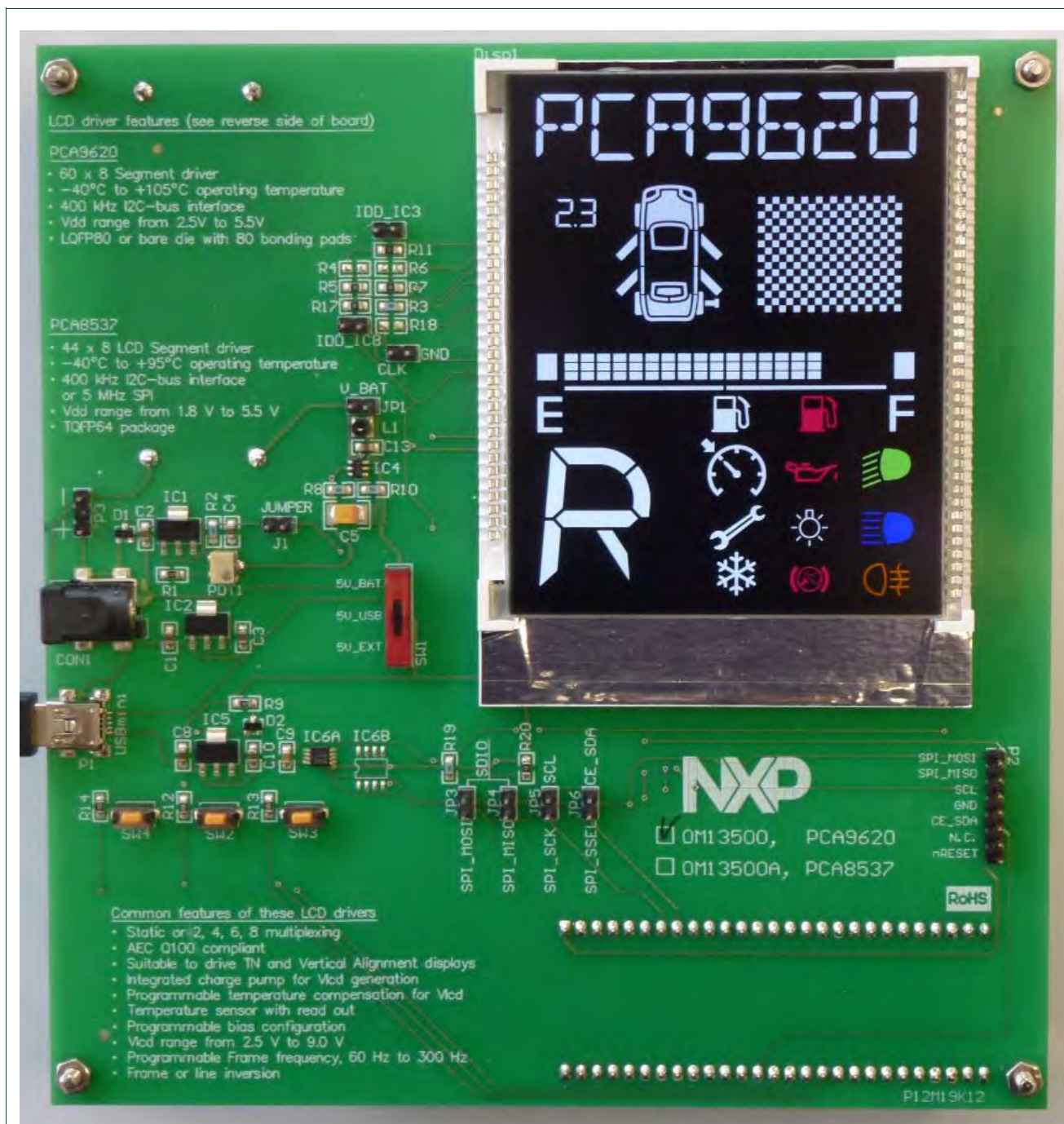
Fig 1. Top view of OM13500 demo board
