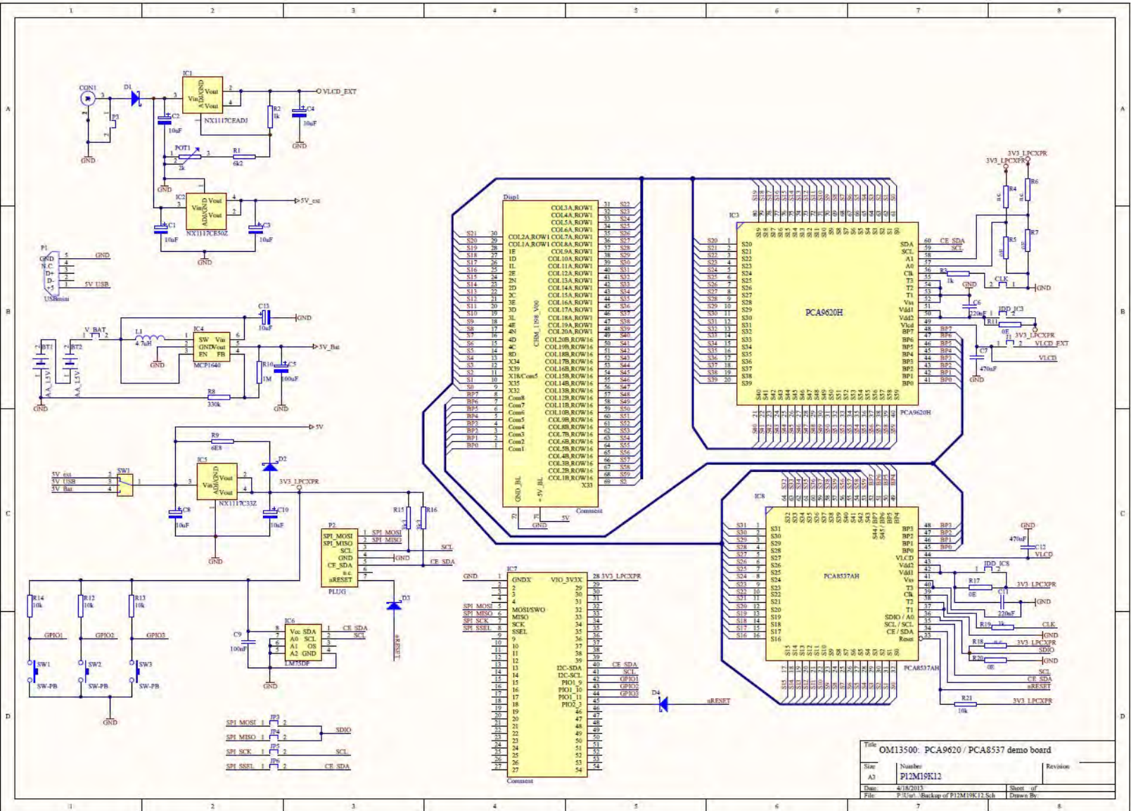
Fig 2. OM13500 schematic
