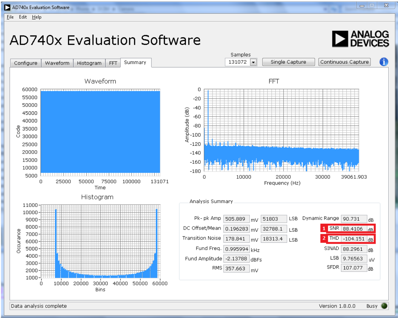
Figure 19. Summary Tab
