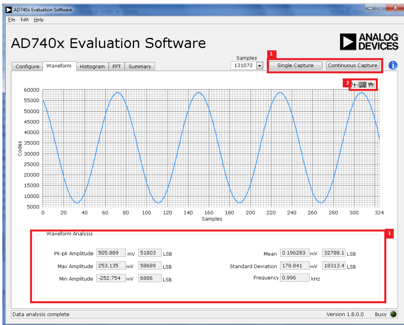
Figure 16. Waveform Capture Tab
