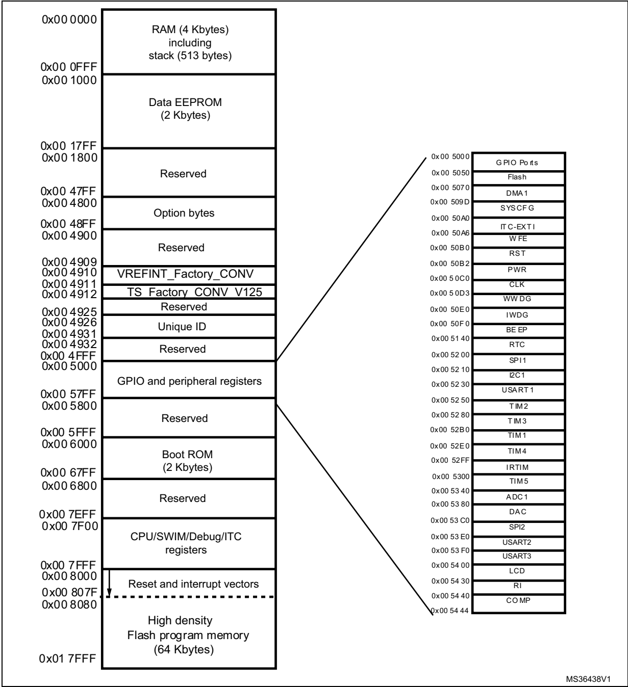
Figure 9. Memory map
