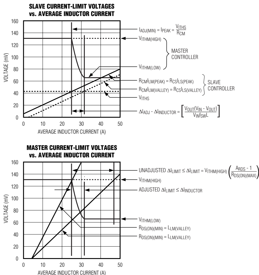
Figure 6. Master/Slave Current-Limit Thresholds
