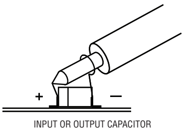
Figure 5. Measuring Input or Output Ripple
