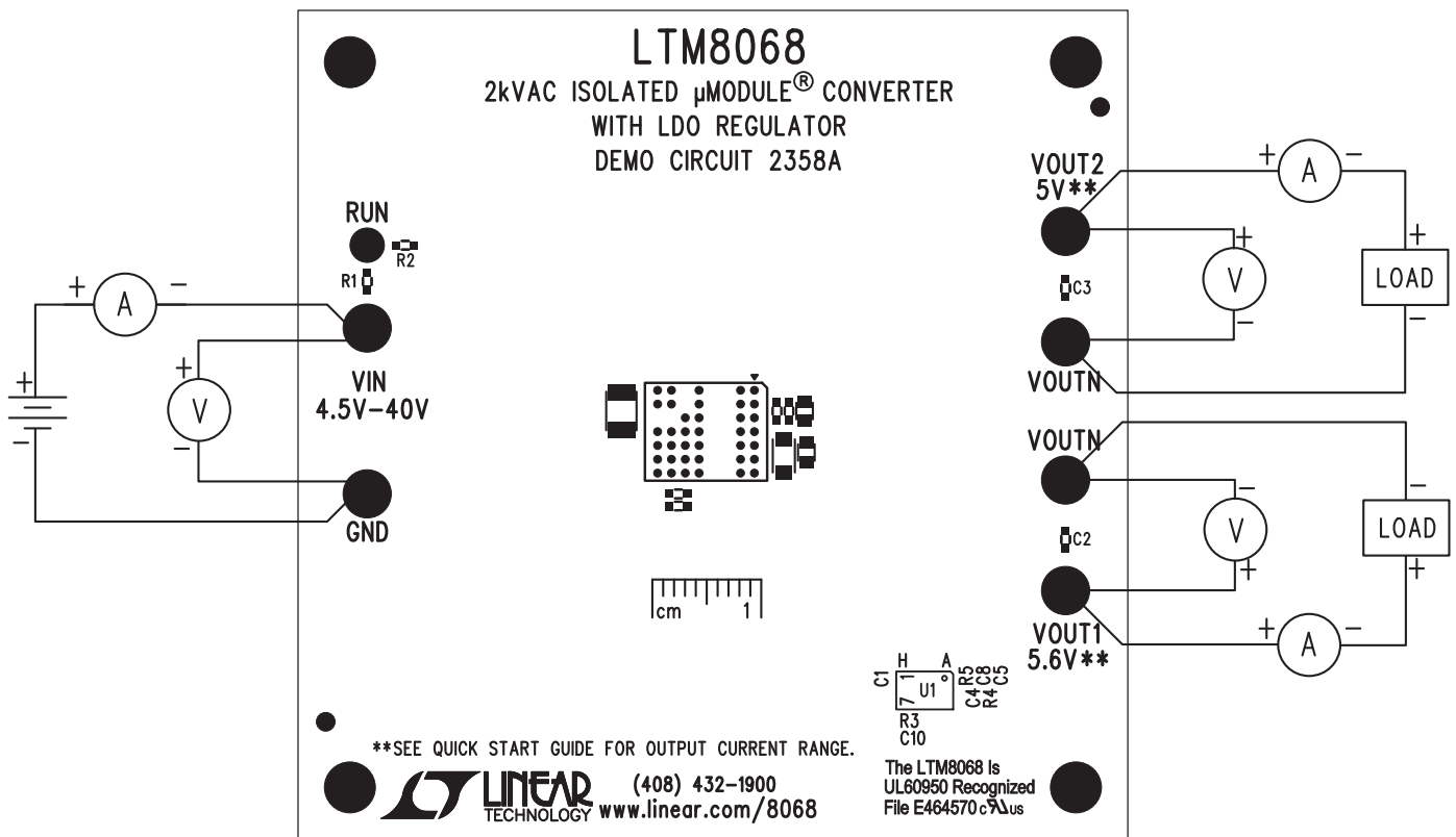
Figure 4. DC2358A Proper Equipment Setup
