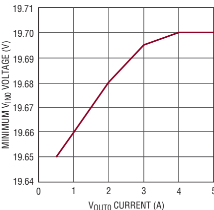
Minimum V_{IN0} vs Output Current, V_{OUT0} = 18\text{V}
