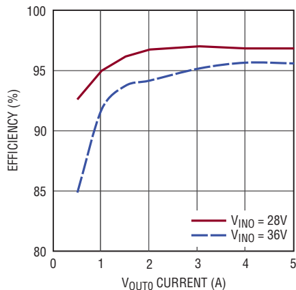
Efficiency vs Output Current, V_{OUT0} = 24\text{V}
