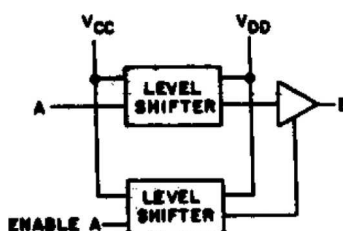
Logic Diagram (1 of 4 Units)
