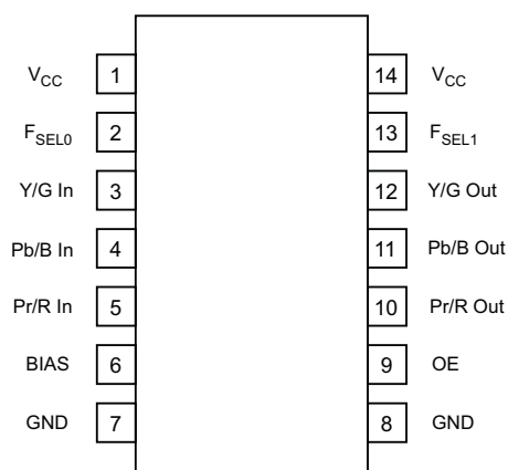
Figure 2. Pin Configuration
