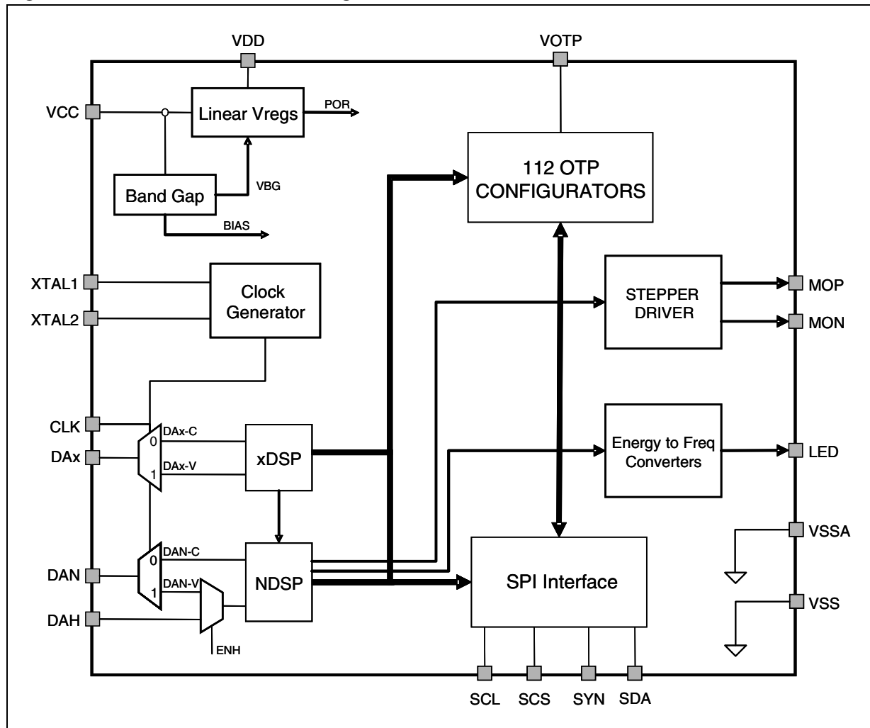
Figure 1. STPMC1 device block diagram
