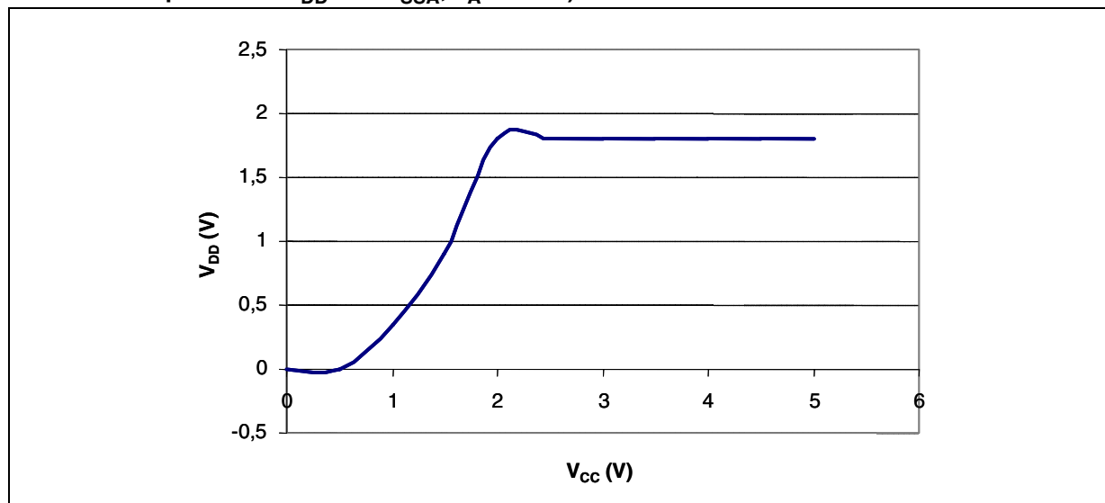
Figure 6. Digital voltage regulator: line - load regulation. ( f_{\text{XTAL1}} = 0 ; 100 nF across V_{CC} and V_{SS} ; 1 \mu\text{F} across V_{DD} and V_{SSA} ; T_A = 25^\circ\text{C} )
