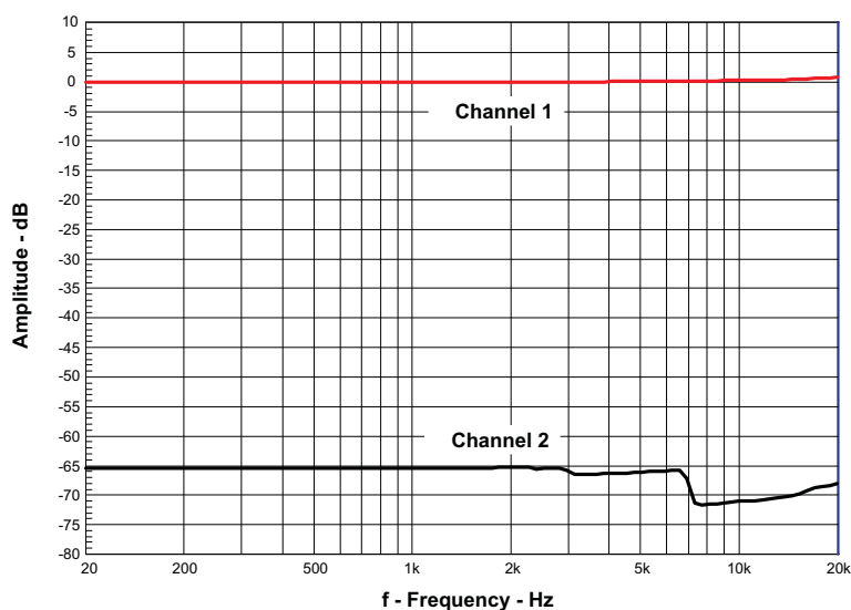
Figure 14. Channel Separation
