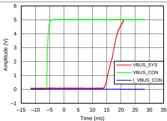
Figure 8. Power Up With 2.2 µF on V BUS_SYS
