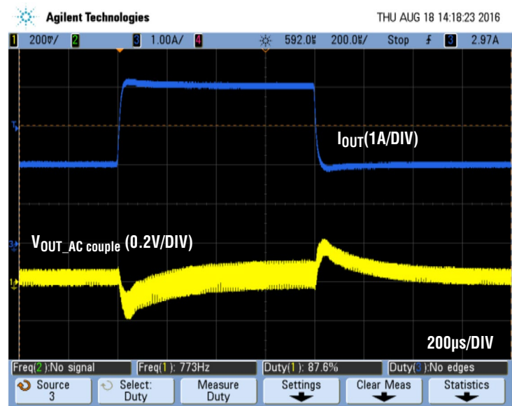
Figure 4. Output Voltage Transient Response, V_{IN} = 12V , V_{OUT} = 12V , I_{OUT} = 2A to 4A to 2A
