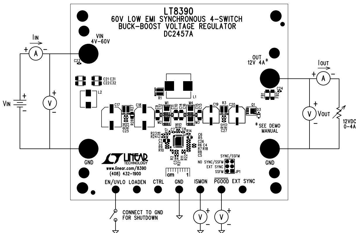
Figure 1. Test Procedure Setup Drawing for DC2457A
