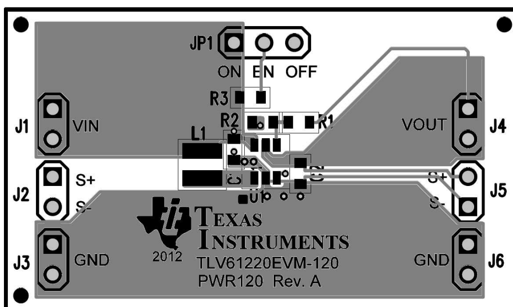
Figure 7. Top Layer
