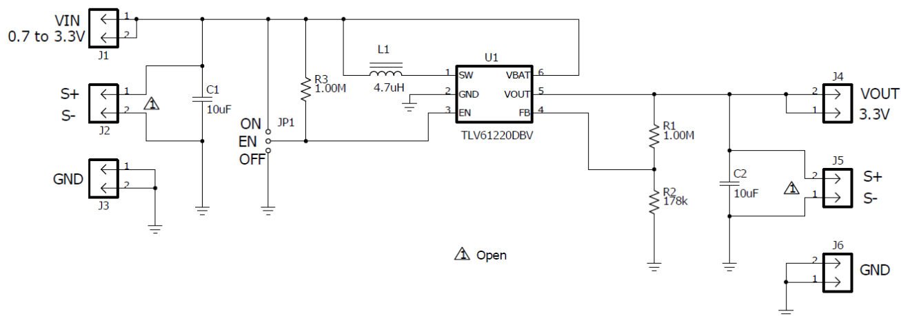
Figure 9. Schematic
