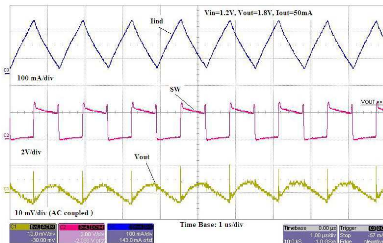
Figure 1. Continuous-Current Operation, TLV61220EVM
