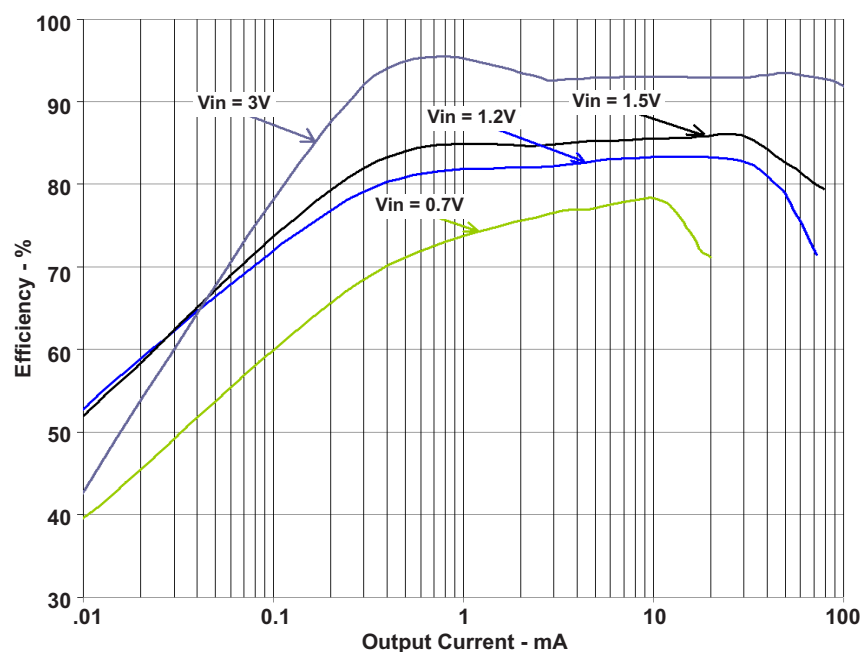
Figure 5. TLV61220 Efficiency
