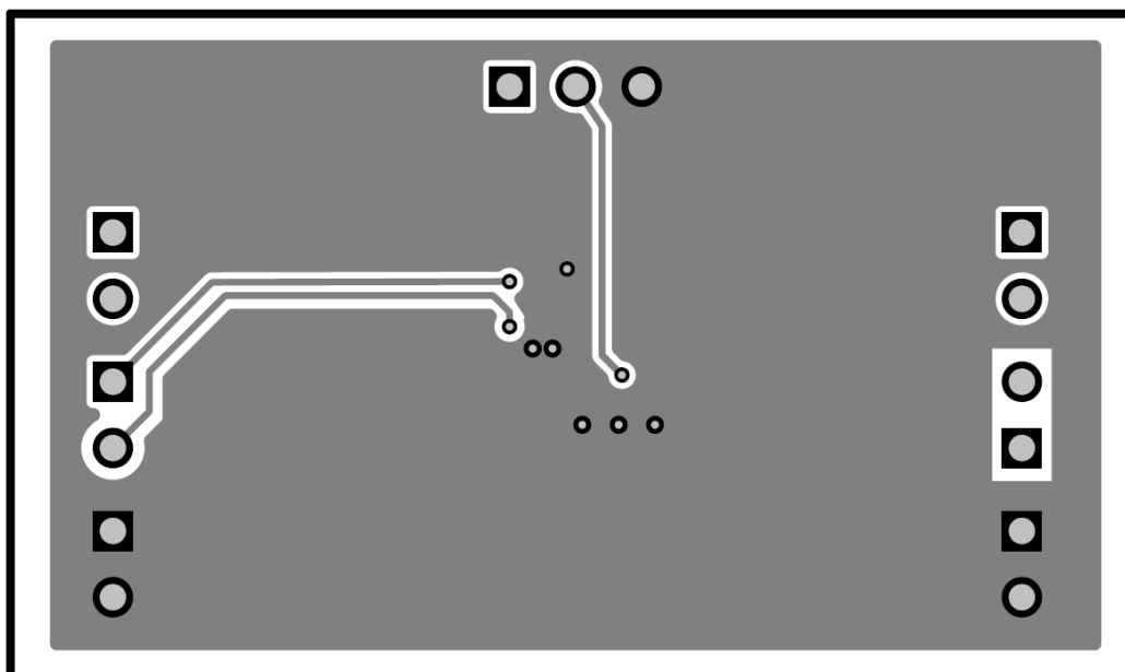
Figure 8. Bottom Layer
