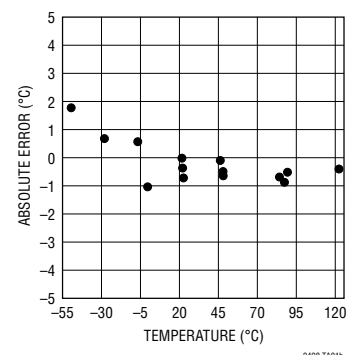
Internal Sensor Absolute Temperature Error
