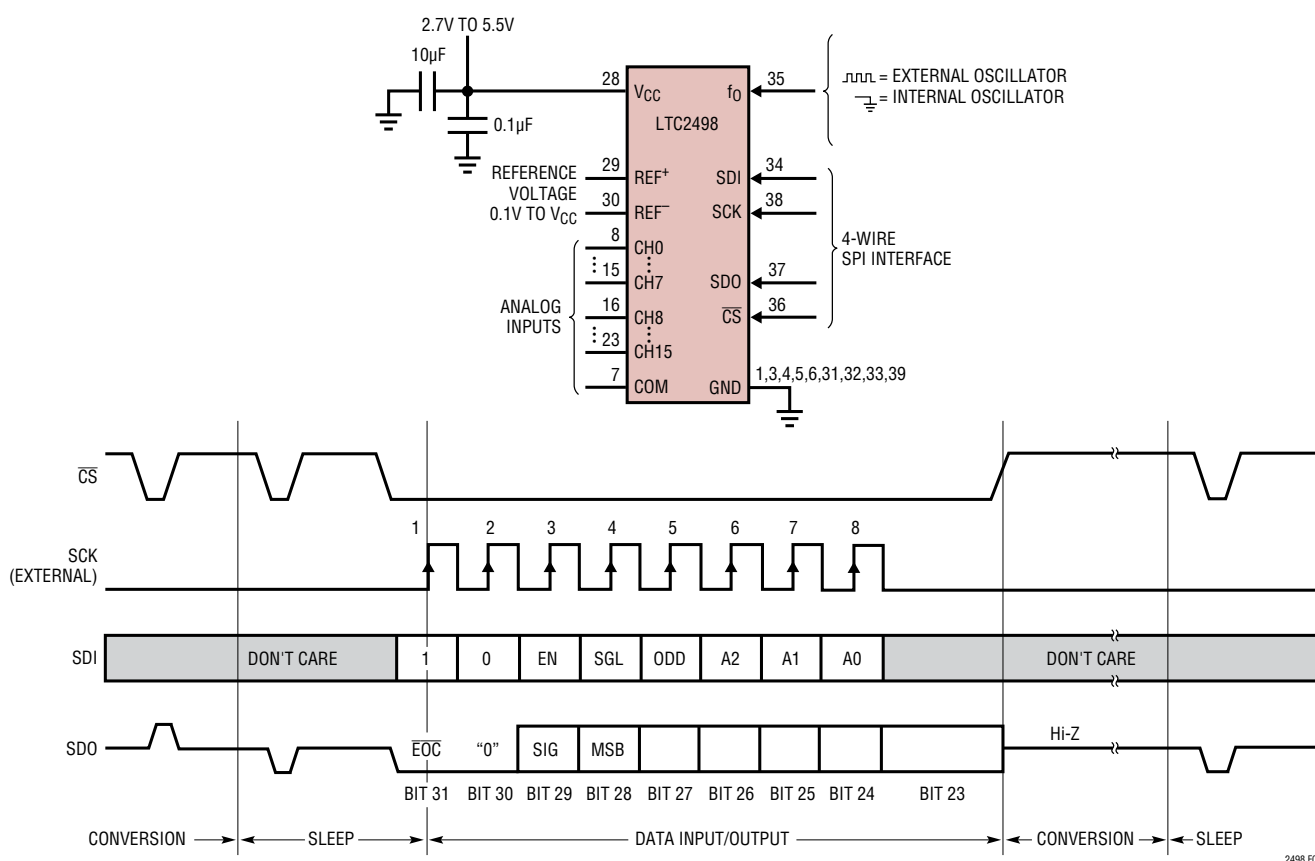
Figure 7. External Serial Clock, Reduced Output Data Length and Valid Channel Selection
