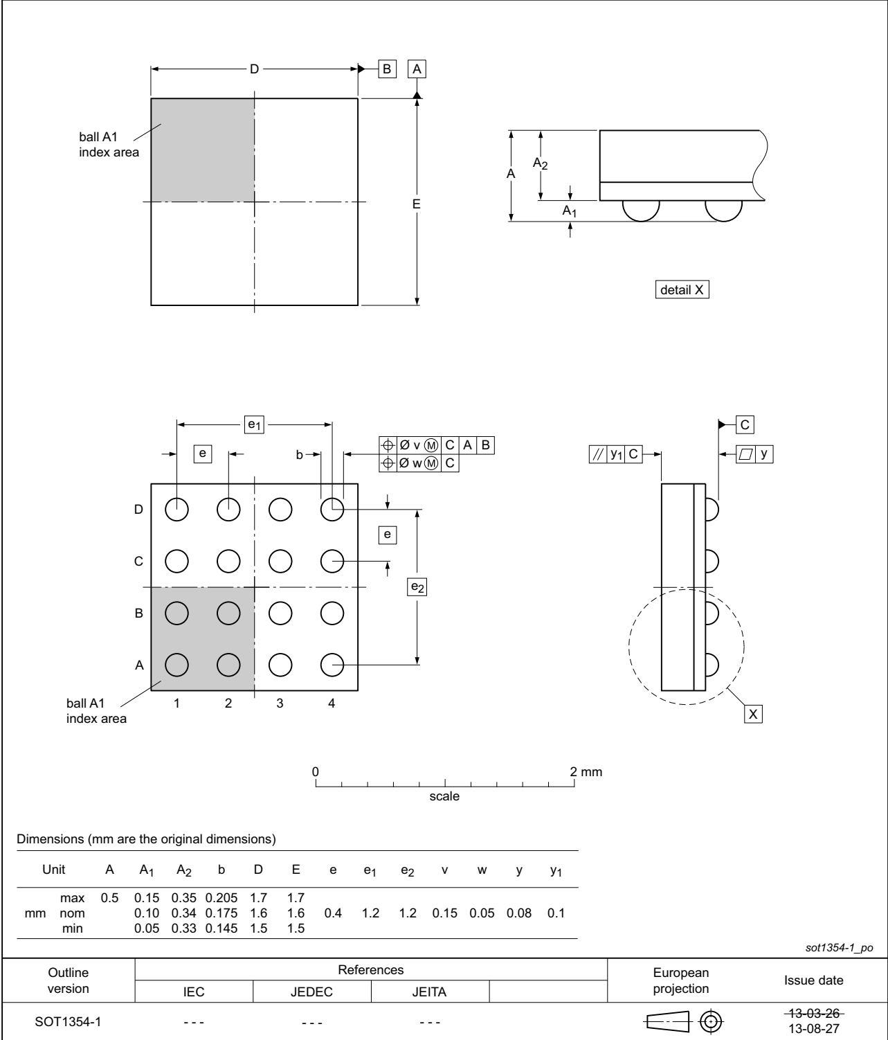
Fig 39. Package outline SOT1354-1 (XFBGA16)
