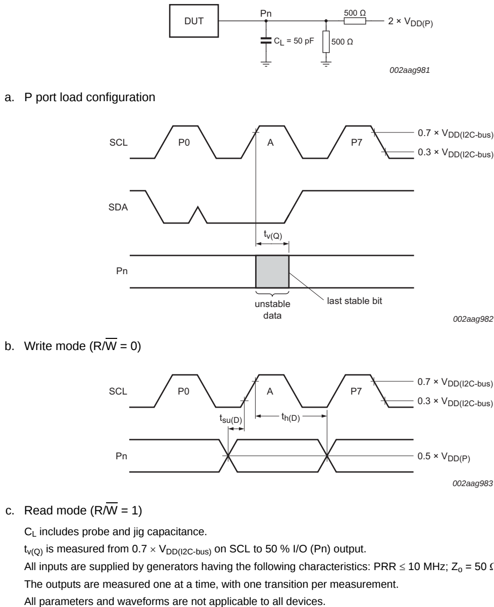
Fig 34. P port load circuit and voltage waveforms
