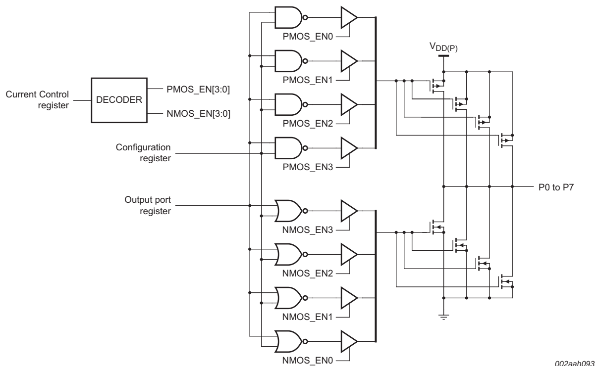
Fig 19. Simplified output stage
