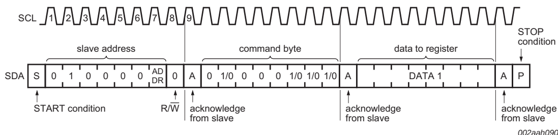
Fig 12. Write to Configuration or Polarity inversion registers
