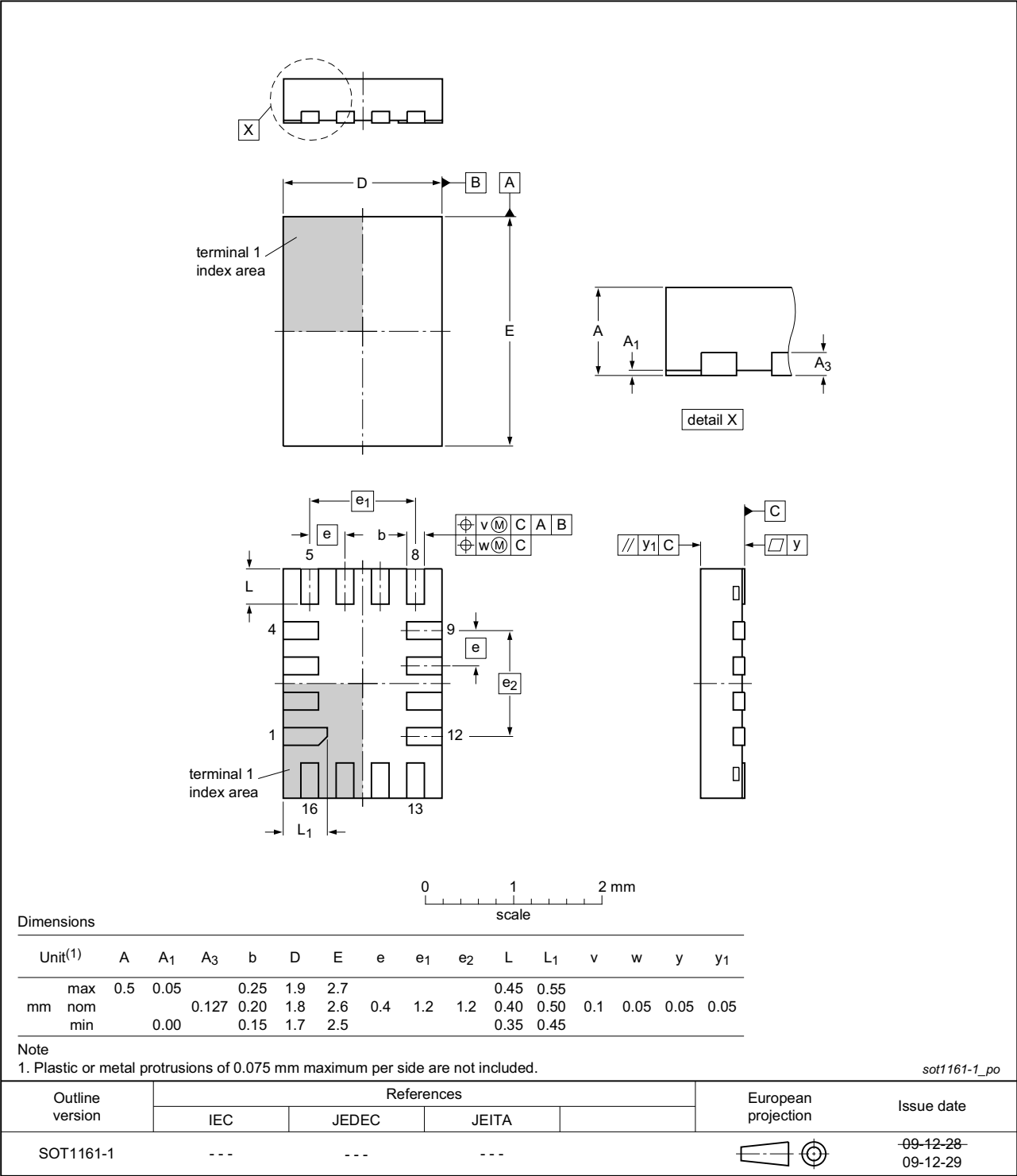
Fig 38. Package outline SOT1161-1 (XQFN16)
