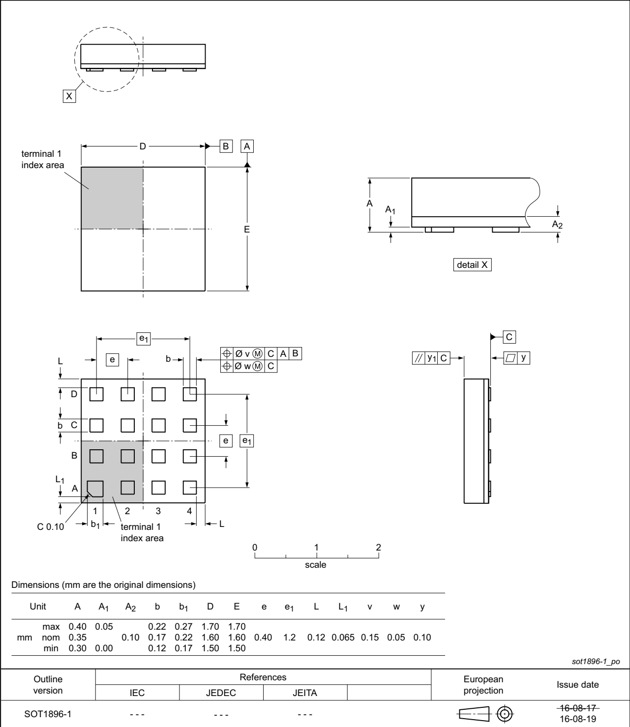
Fig 40. Package outline SOT1896-1 (X2QFN16)
