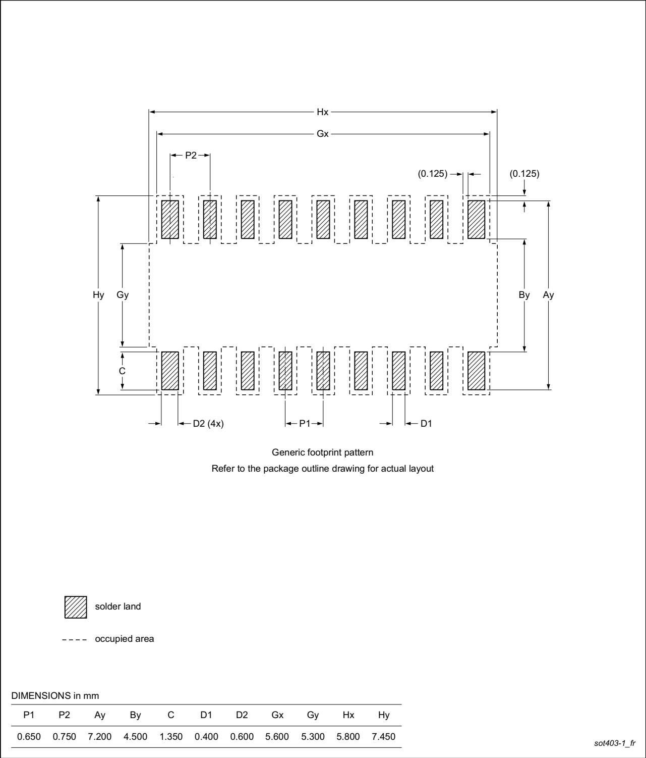
Fig 43. PCB footprint for SOT403-1 (TSSOP16); reflow soldering
