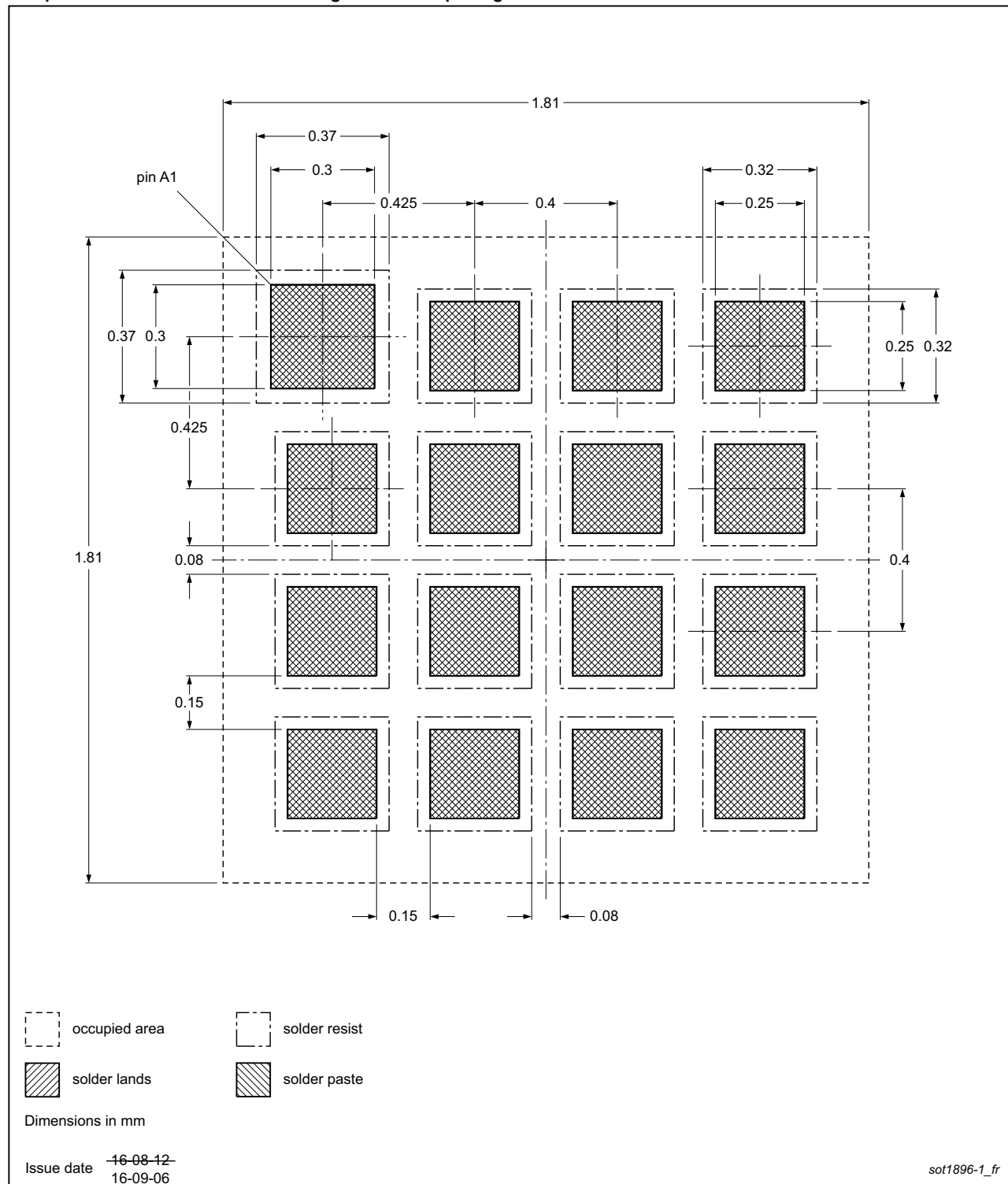
Fig 45. PCB footprint for SOT1896-1 (X2QFN16); reflow soldering
