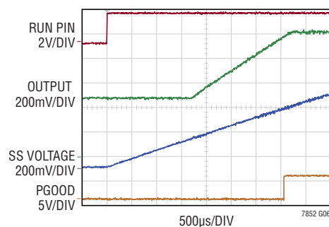
Prebias Startup at 0.5V
