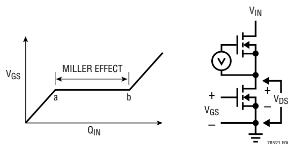
Figure 6. Gate Charge Characteristic
