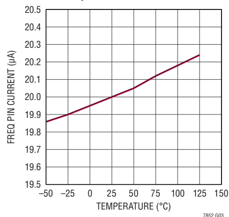
FREQ Pin Source Current vs Temperature
