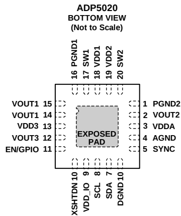
Figure 4. Pin Configuration (Bottom View)
