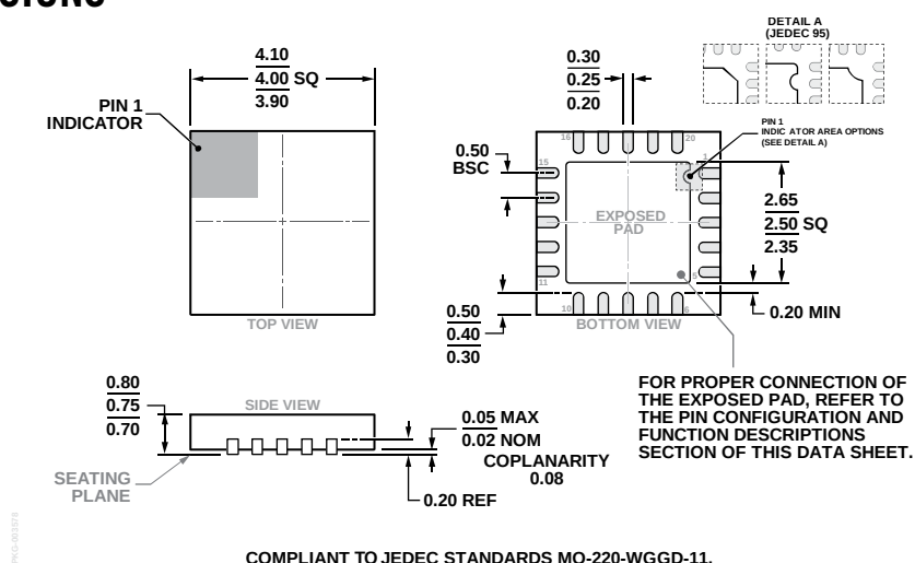
Figure 30. 20-Lead Lead Frame Chip Scale Package [LFCSP] 4 mm × 4 mm Body and 0.75 mm Package Height (CP-20-10) Dimensions shown in millimeters
