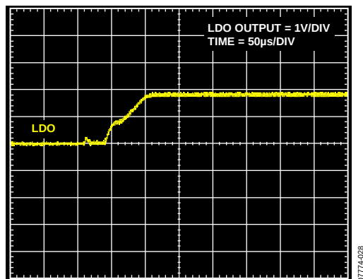
Figure 18. LDO Startup
