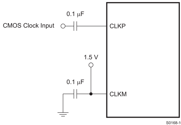
Figure 69. Single-Ended Clock Driving Circuit
