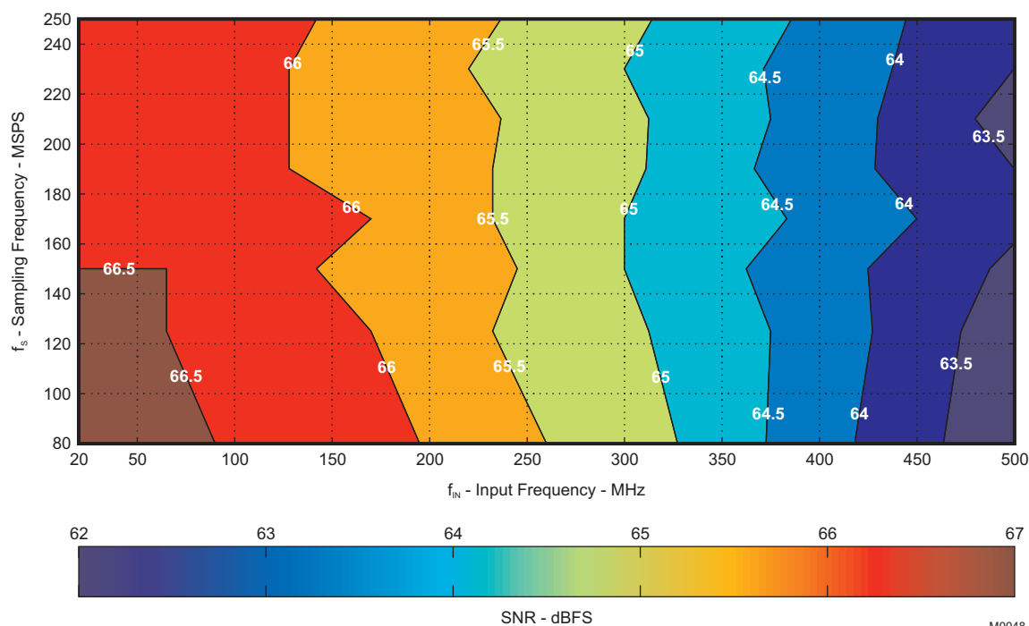
Figure 60. SNR Contour Plot (6-dB gain)
