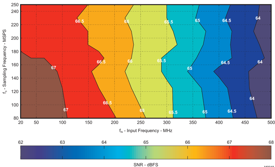
Figure 58. SNR Contour Plot (6-dB gain)
