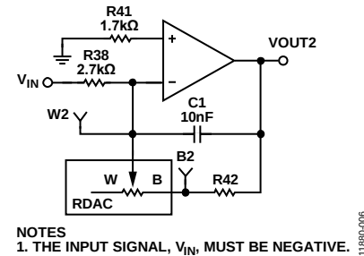
Figure 6. Inverting Amplifier with Linear Gain
