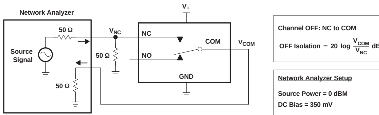
Figure 12. OFF Isolation ( O_{\text{ISO}} )
