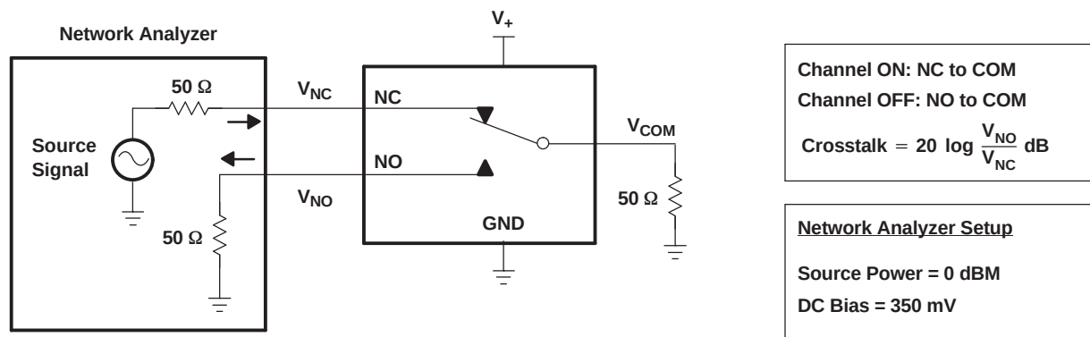
Figure 13. Crosstalk ( X_{\text{TALK}} )
