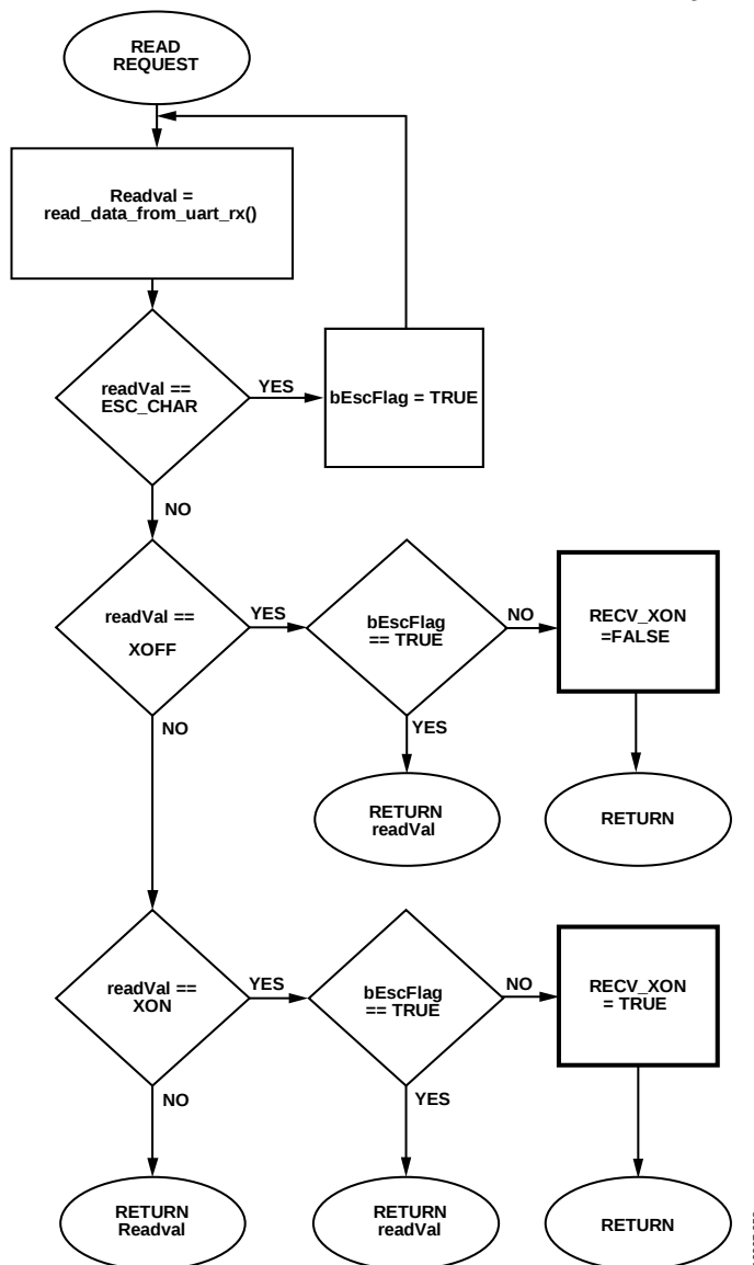
Figure 44. Flowchart of the Control Signals in the ISR Being Processed
