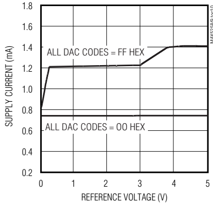
SUPPLY CURRENT vs. REFERENCE VOLTAGE ( V_{DD} = +5V )
