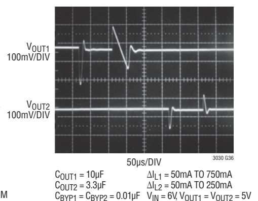
Channel-to-Channel Isolation
