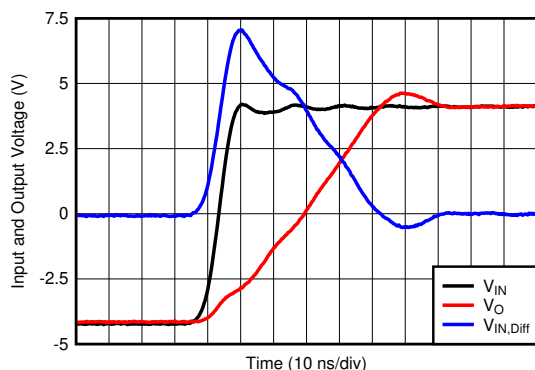
Figure 78. Large-Signal Transient Response Using OPA2810
