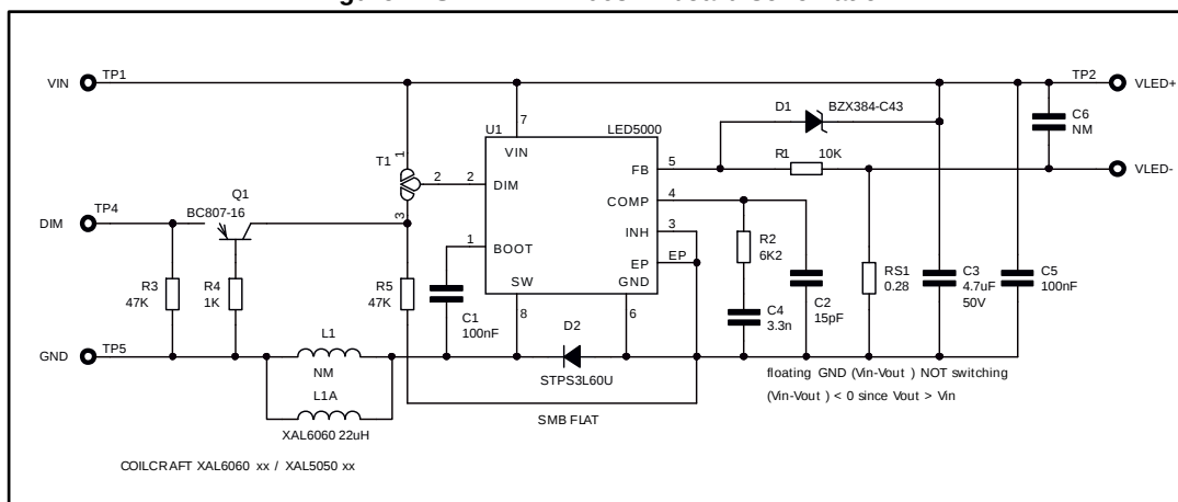
Figure 1: STEVAL-ILL063V1 board schematic
