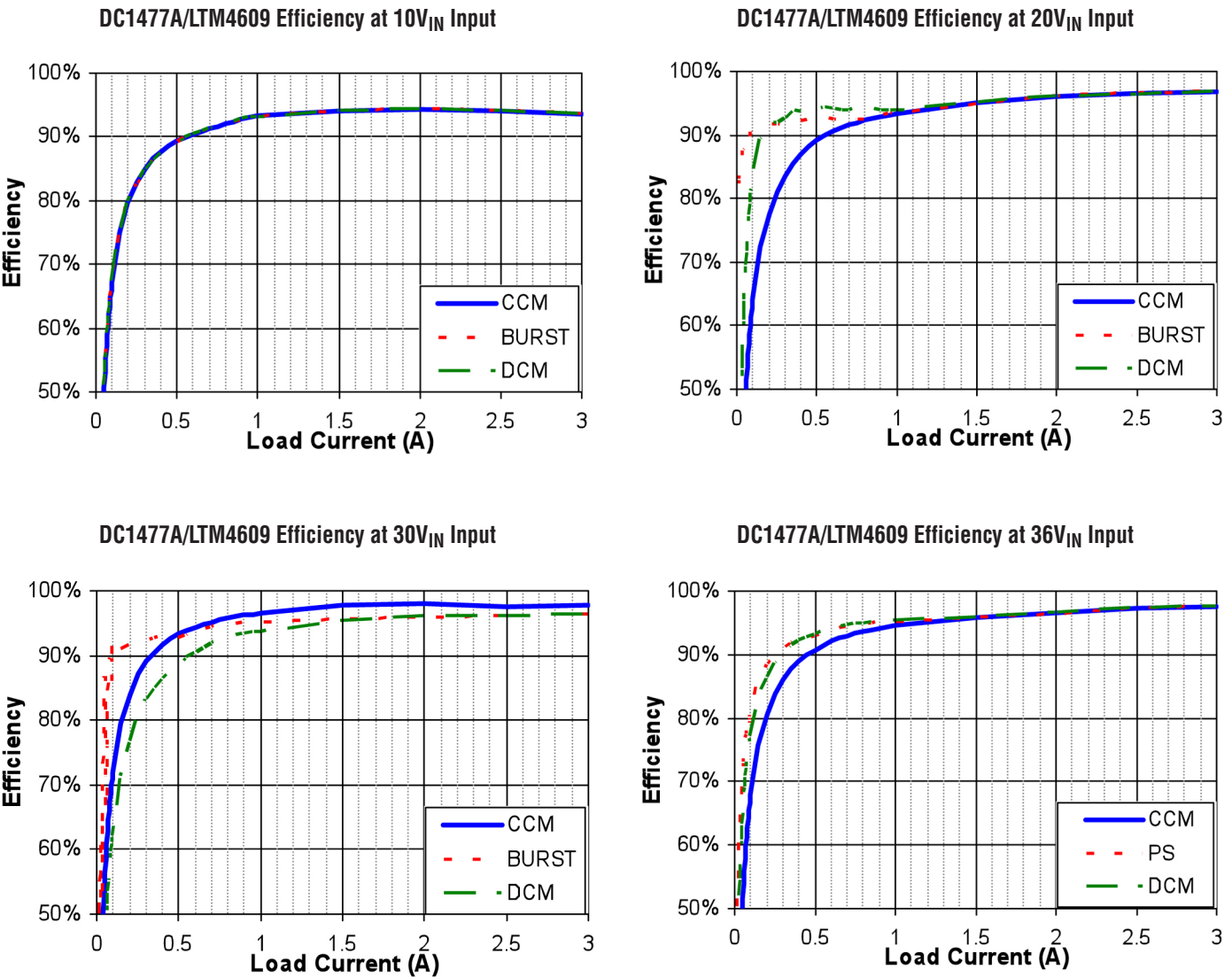
Figure 3. Measured Efficiency at Different V IN
