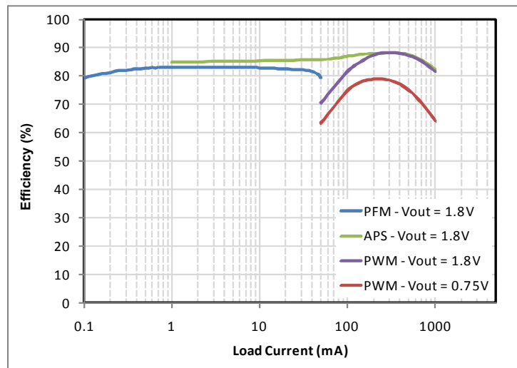
Figure 22. SW4 Efficiency Waveforms
