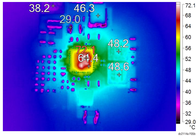
Figure 5. Thermal Image Top View, IOUT1 = 1A, IOUT2 = 1A, IOUT3 = 1.5A, TA = 25°C, fSW = 2MHz
