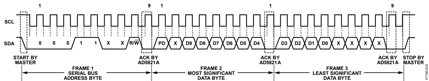
Figure 23. Read Operation
