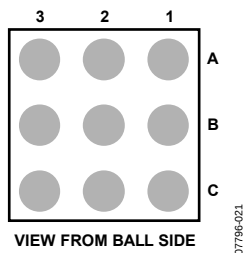
Figure 3. Pin Configuration
