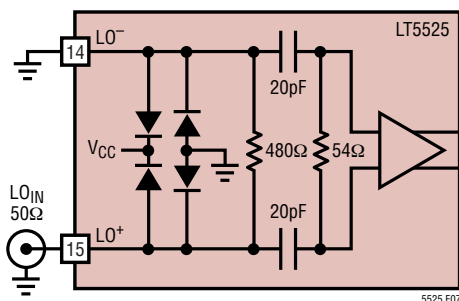
Figure 7. LO Input Schematic
