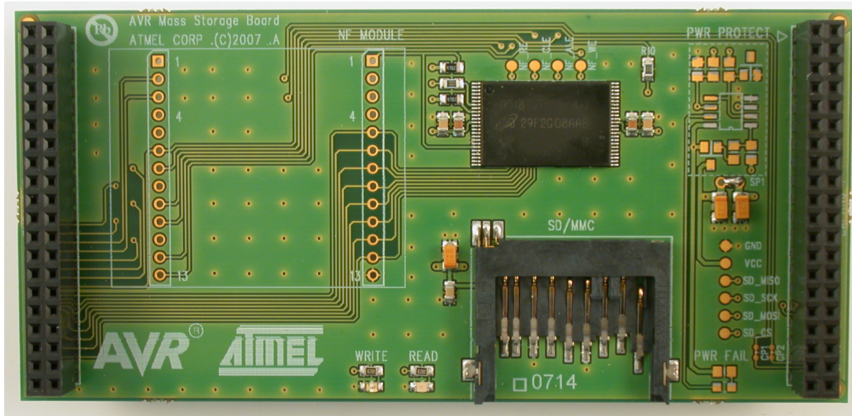
Figure 1-1 . ATEVK525
