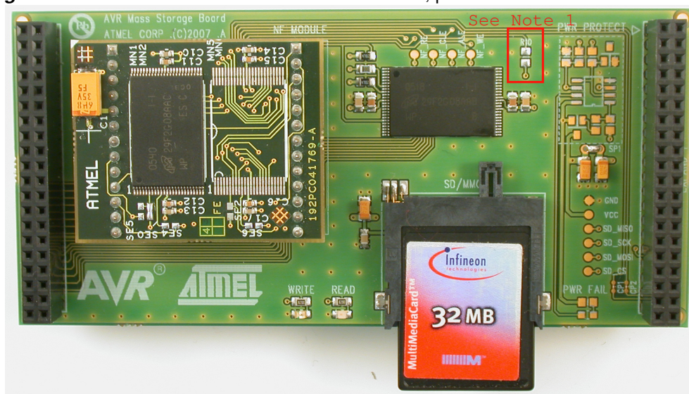
NF Module Installation Figure 2-5 . NAND Flash module on the ATEVK525, plus MMC card
