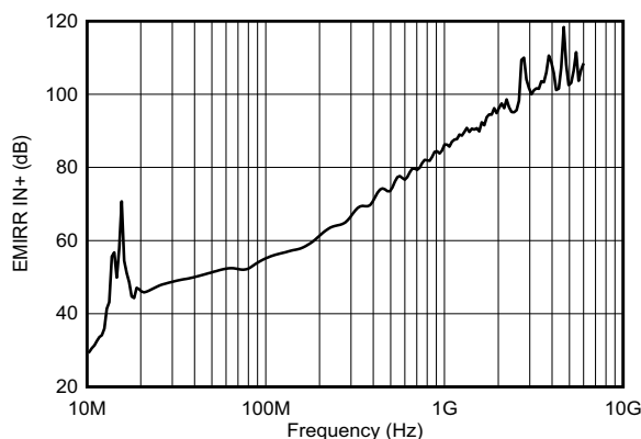
Figure 46. OPA207 EMIRR IN+ vs Frequency
